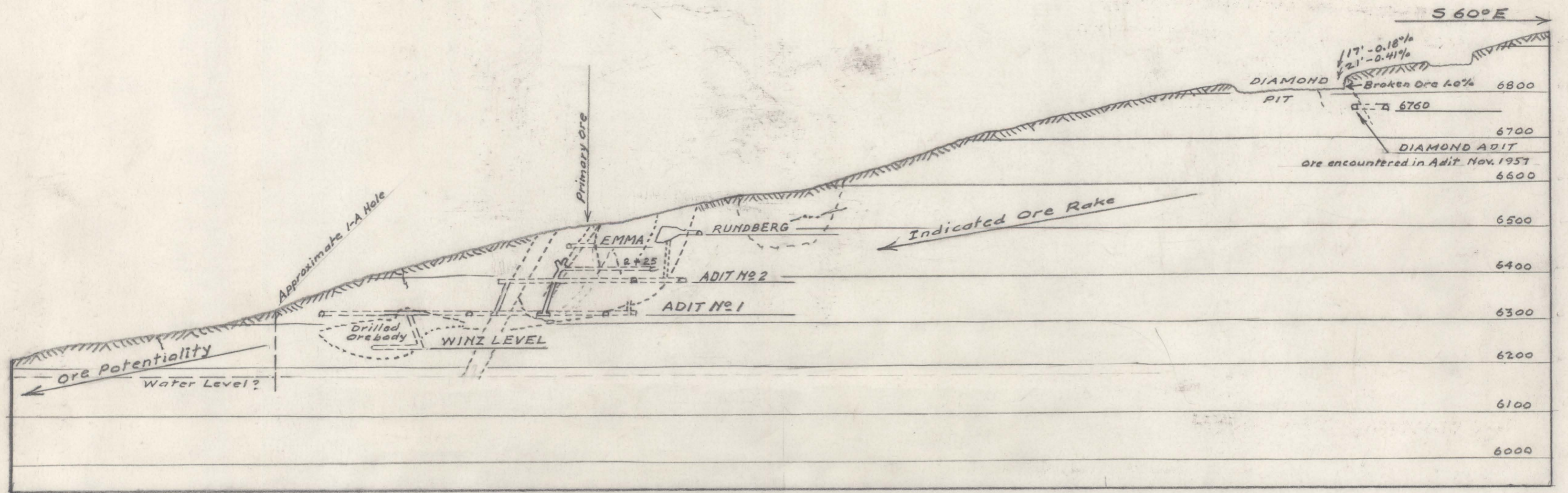
GENERALIZED LONGITUDINAL SECTION SCALE: 200-ft. to 1-in.
