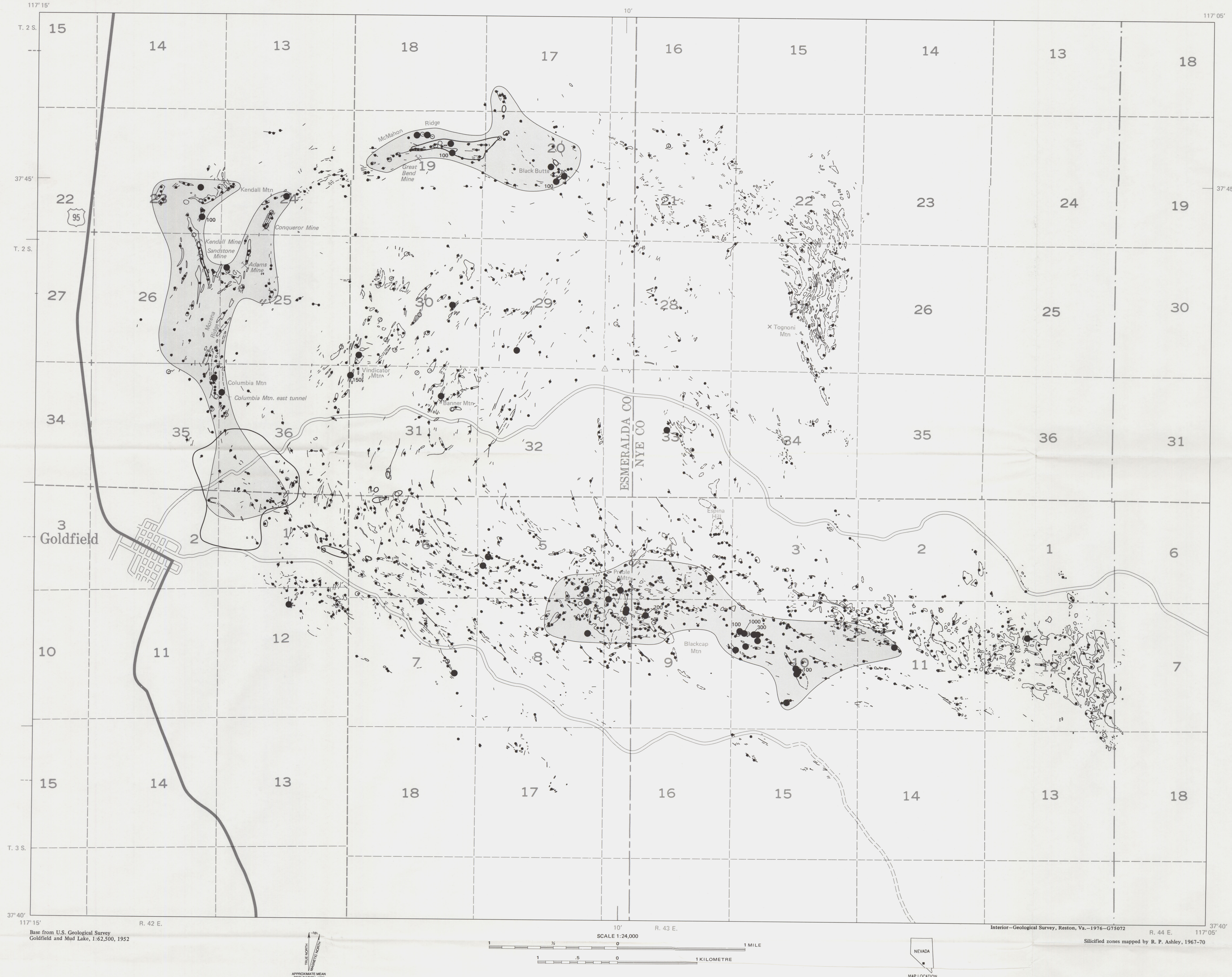
GEOCHEMICAL MAP SHOWING DISTRIBUTION AND ABUNDANCE OF BISMUTH IN SILICIFIED ROCKS, GOLDFIELD MINING DISTRICT, ESMERALDA AND NYE COUNTIES, NEVADA
