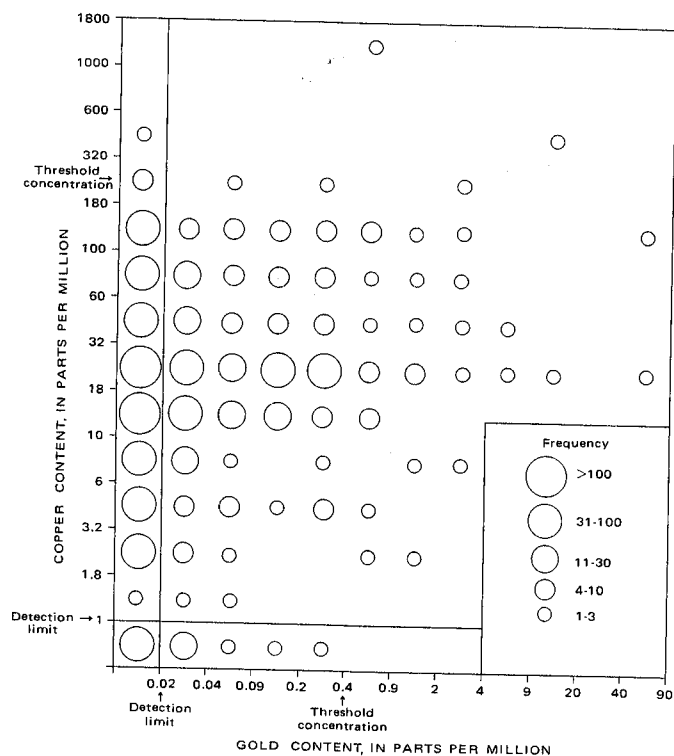
FIGURE 7.—Bivariate frequency distribution of gold and copper.
