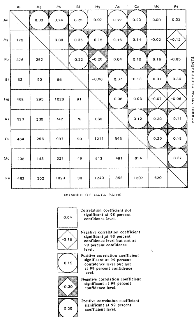
FIGURE 6.—Spearman correlation matrix for total data set (1,337 samples).
