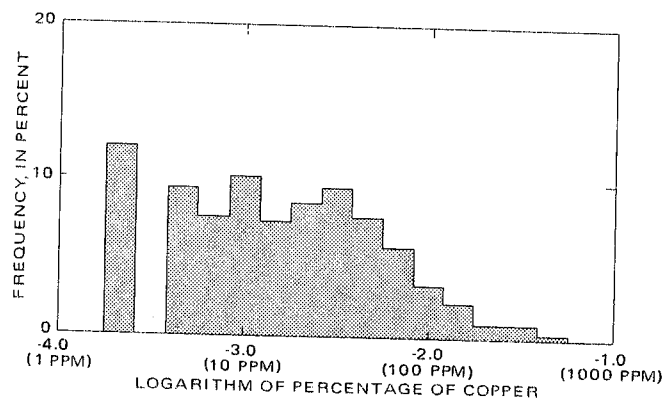
FIGURE 5.—Copper content of 323 silicified rock samples.
