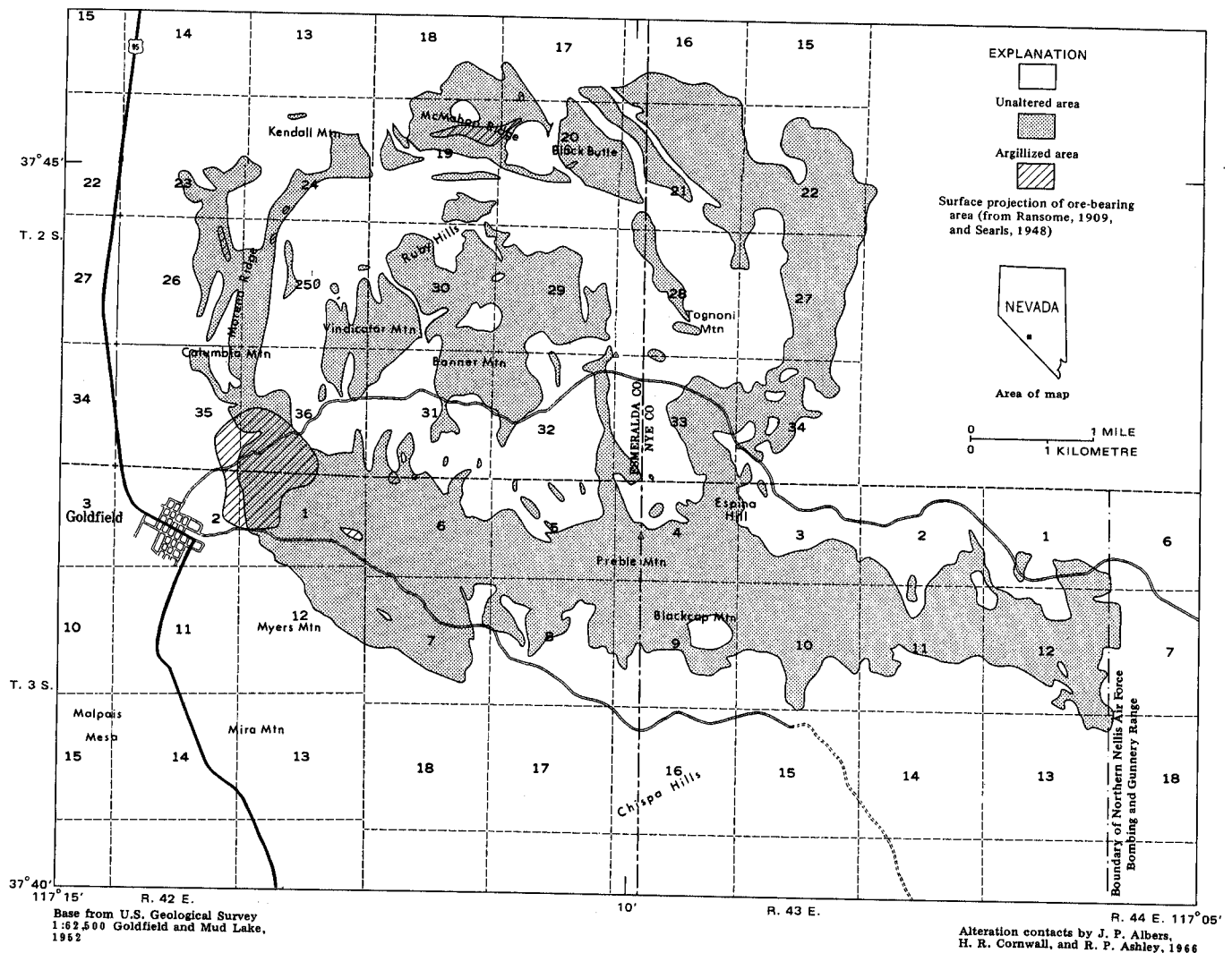
FIGURE 1.—Map of Goldfield and vicinity showing areas of hydrothermal alteration and ore deposits.
