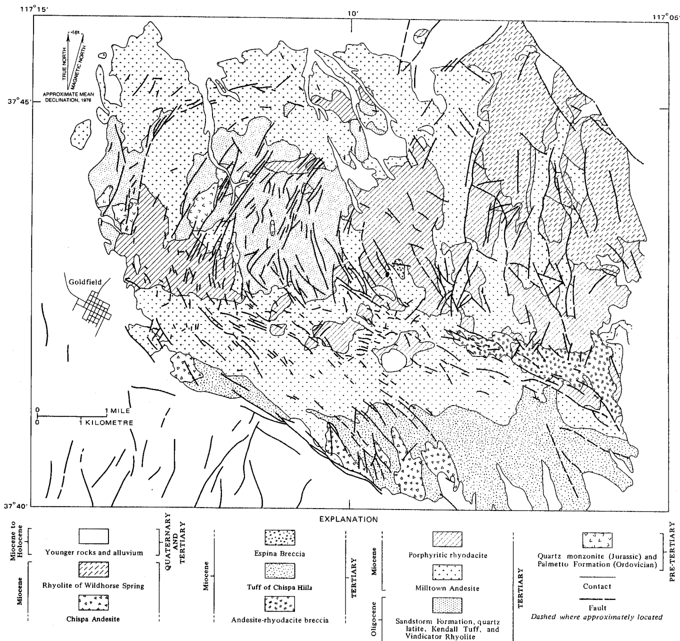
FIGURE 2.—Generalized geologic map of the Goldfield mining district. Modified from Ashley, 1975.
