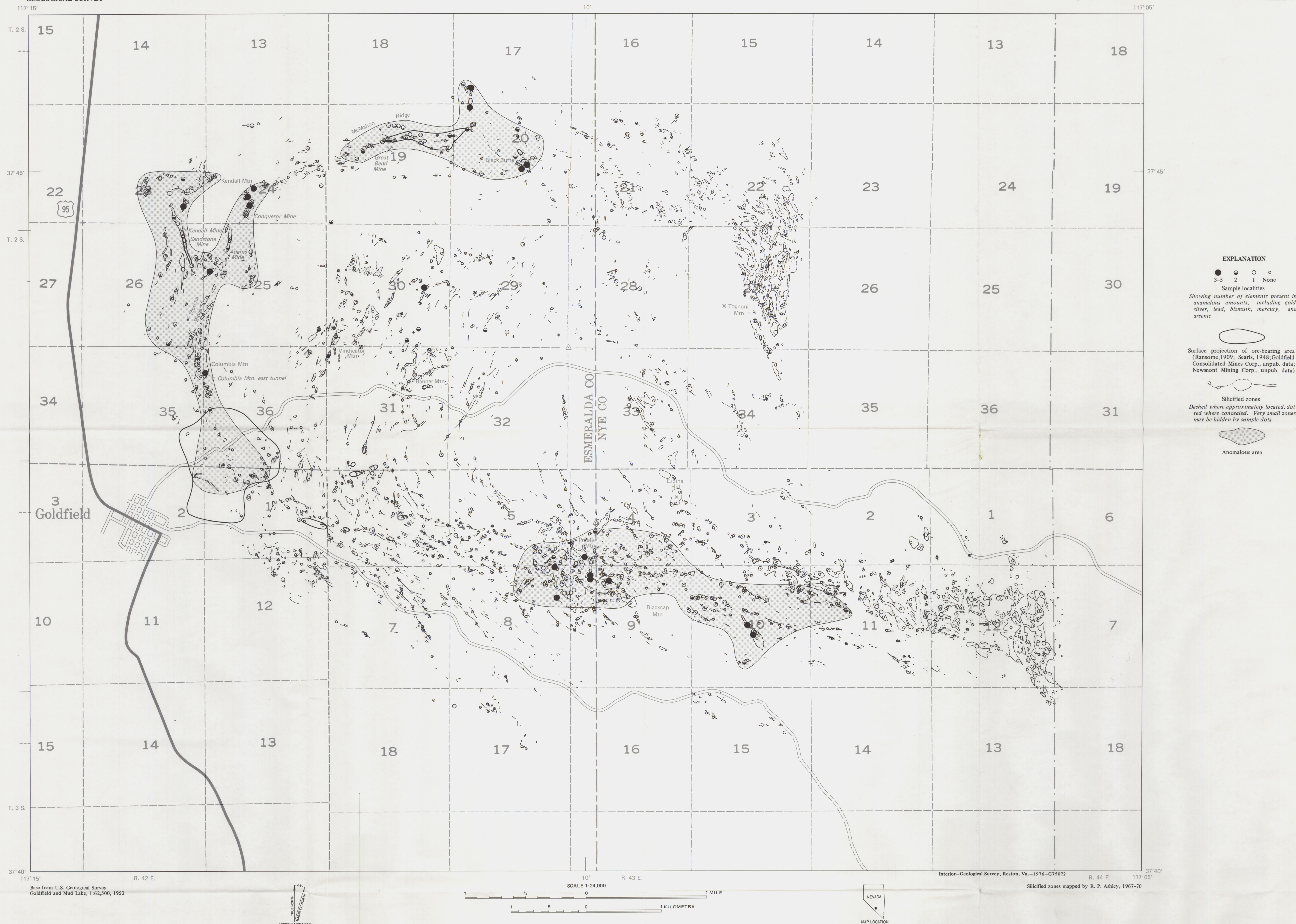
COMPOSITE GEOCHEMICAL MAP SHOWING DISTRIBUTION AND ABUNDANCE OF ELEMENTS IN SILICIFIED ROCKS, GOLDFIELD MINING DISTRICT, ESMERALDA AND NYE COUNTIES, NEVADA
