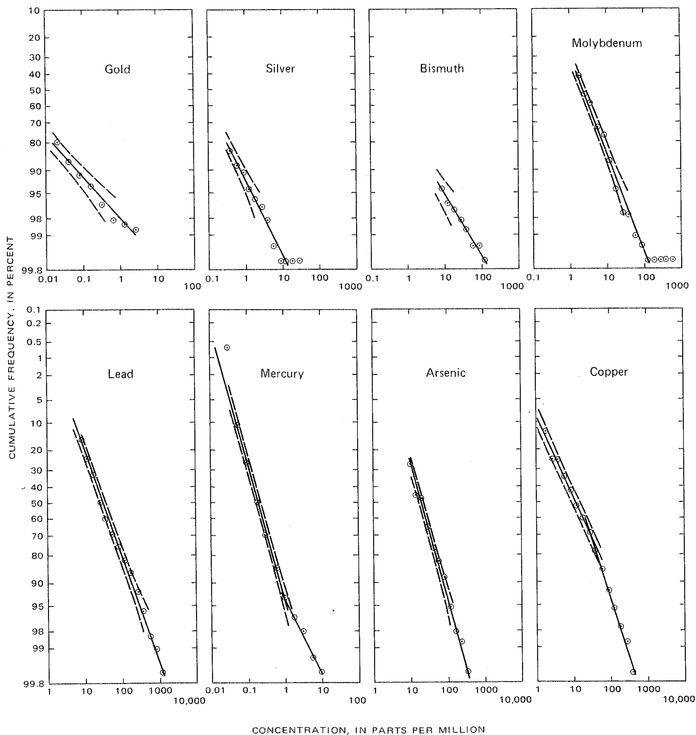
FIGURE 4.—Log-probability plots for gold, silver, bismuth, lead, molybdenum, mercury, arsenic, and copper in 323 silicified rocks. Each data point shows cumulative frequency at the lower end of each class interval. Dashed lines show 95 percent confidence limits for the straight line fit to the data points.
