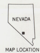
GEOCHEMICAL MAP SHOWING DISTRIBUTION AND ABUNDANCE OF ARSENIC IN SILICIFIED ROCKS, GOLDFIELD MINING DISTRICT, ESMERALDA AND NYE COUNTIES, NEVADA
