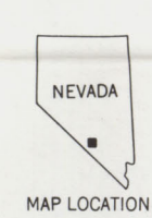
GEOCHEMICAL MAP SHOWING DISTRIBUTION AND ABUNDANCE OF SILVER IN SILICIFIED ROCKS, GOLDFIELD MINING DISTRICT, ESMERALDA AND NYE COUNTIES, NEVADA
