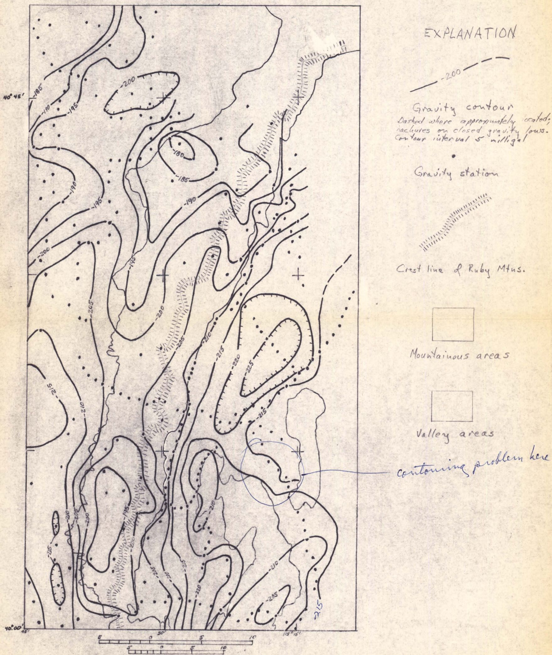
Figure 2. Bouguer anomaly map of Ruby Mountains and adjacent areas.
