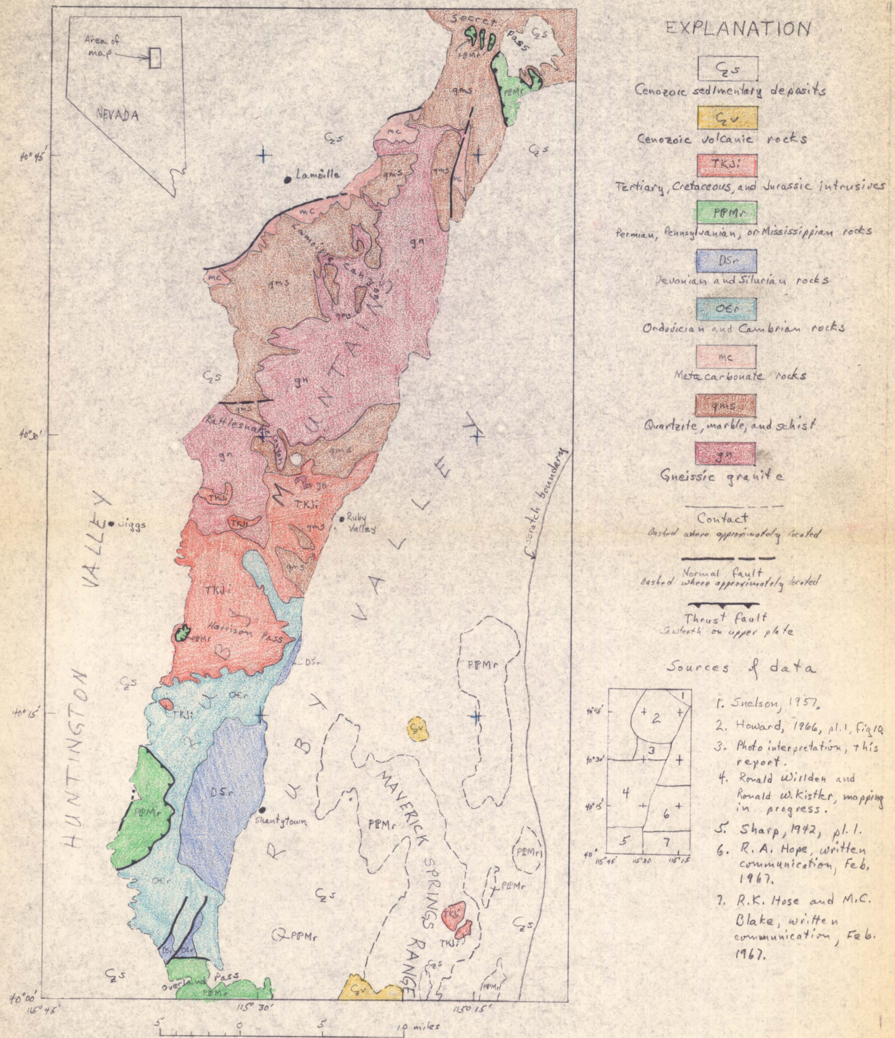
Figure 1. Generalized geologic map of the Ruby Mountains and adjacent areas.
