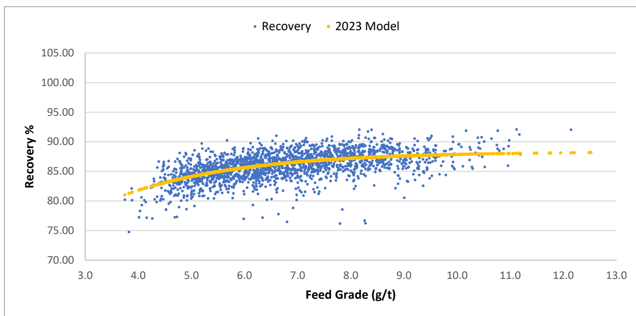
Figure 13-11 Goldstrike Roaster Shift Recovery vs. Feed Grade
