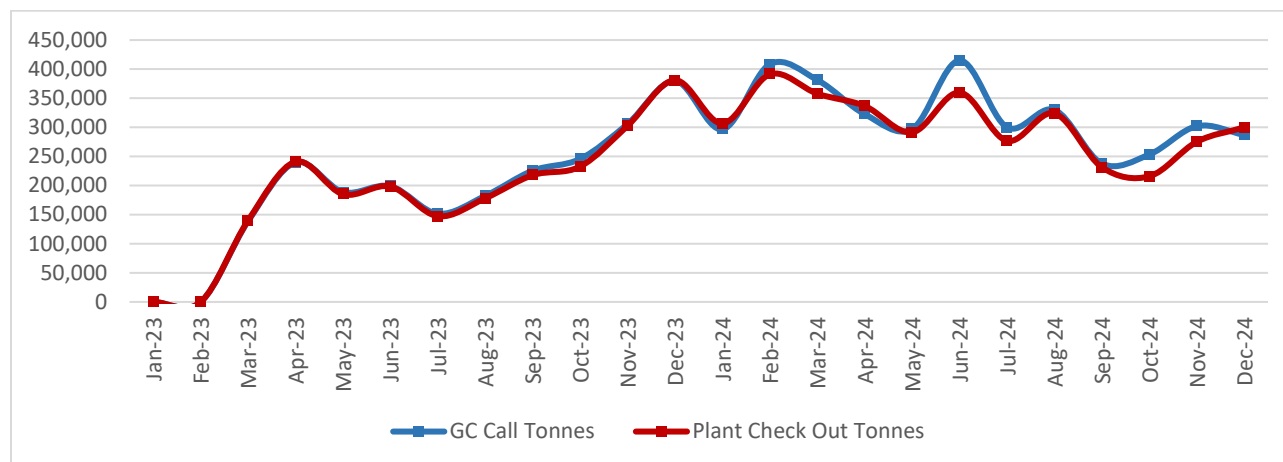
Figure 15-15 Goldstrike Autoclave Monthly Tonnage Comparison
