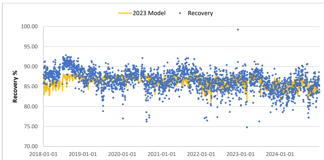
Figure 13-10 Goldstrike Roaster Shift Recovery vs. 2023 Recovery Model
