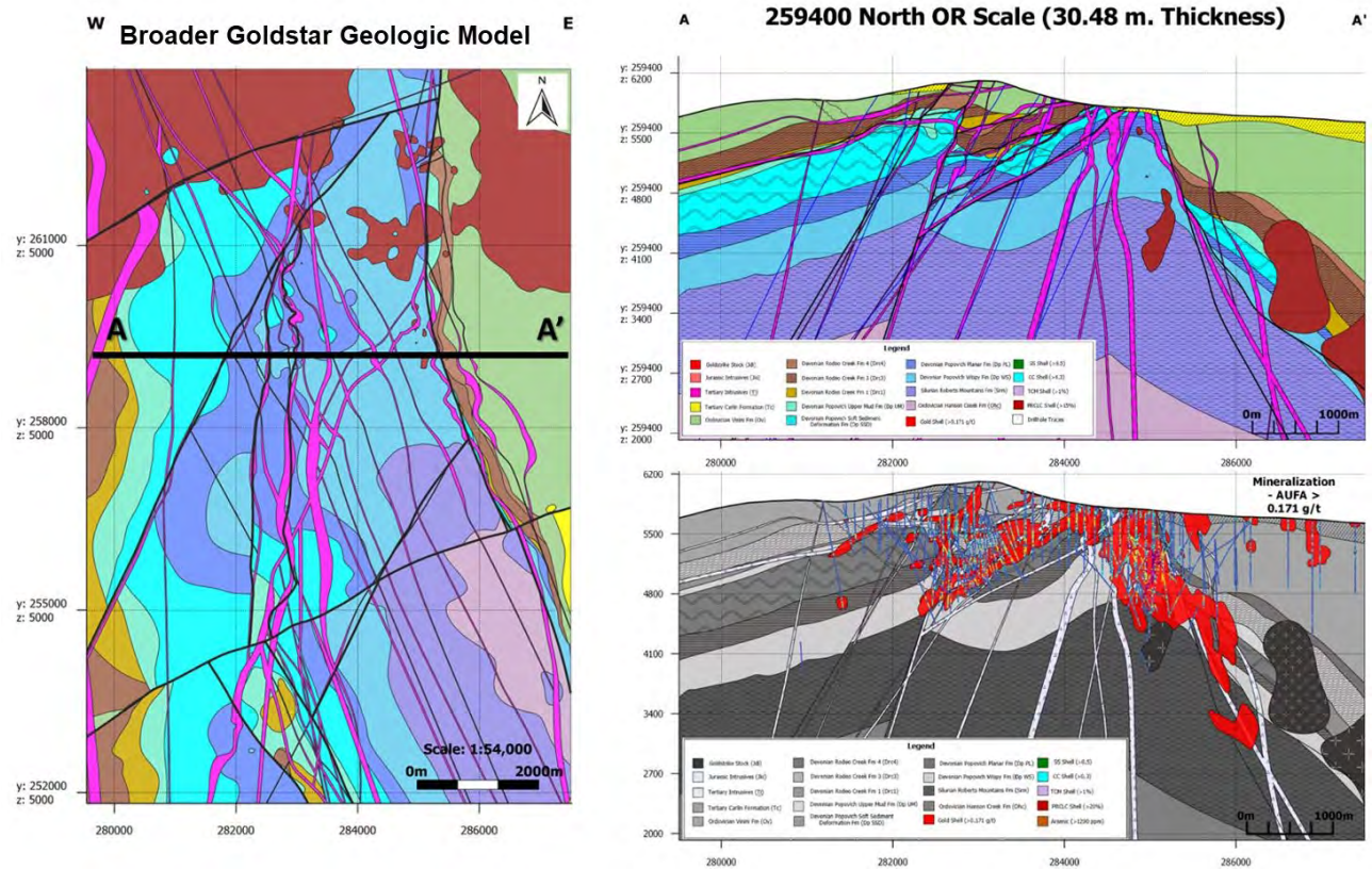
Figure 7-5 Representative Geological Cross-section of the Goldstar Deposit.
