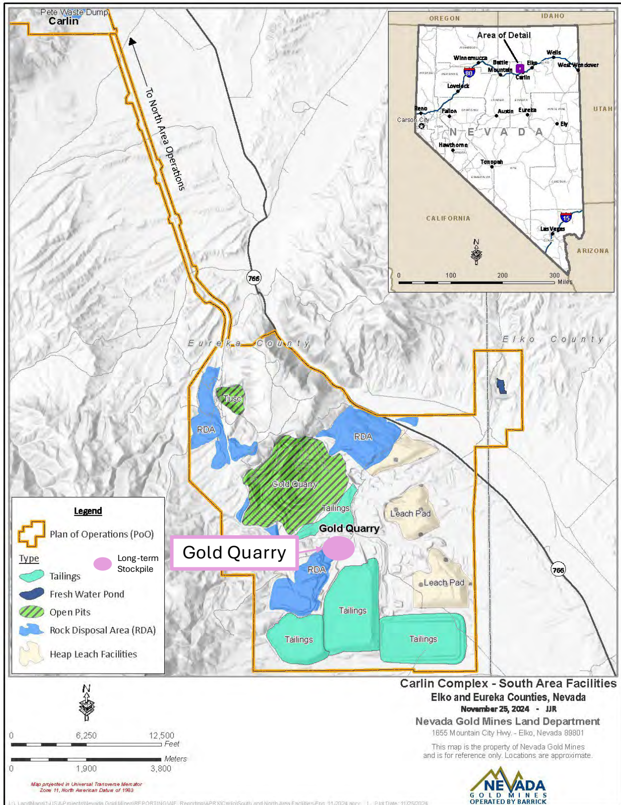
Figure 13-7 Long-term SP Location, Gold Quarry Area
