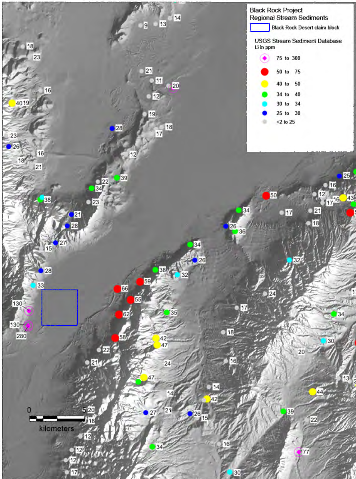
Figure 9 Black Rock Desert Project District Stream Sediments
