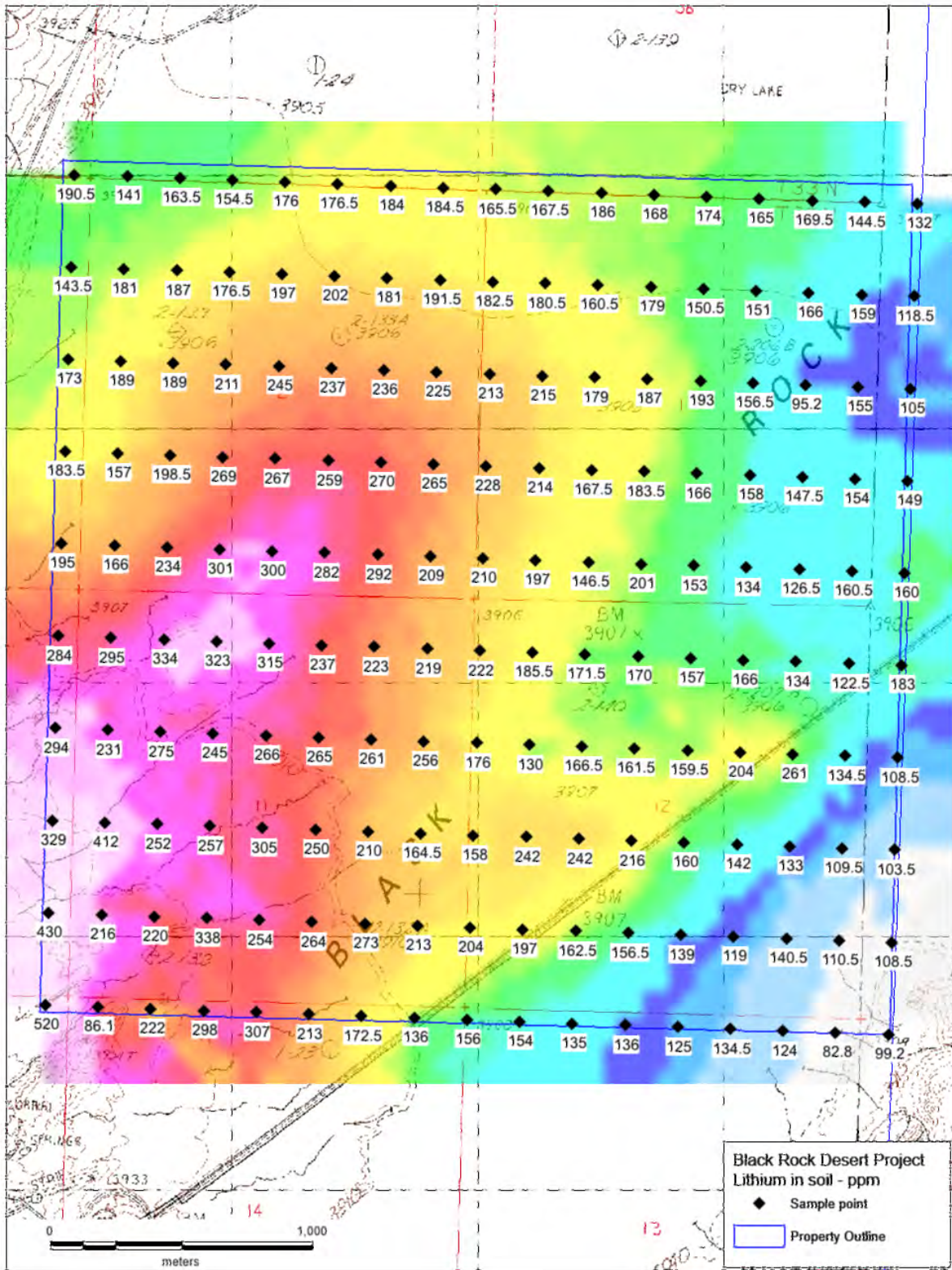
Figure 10 Black Rock Desert Project: grid soil sampling results
