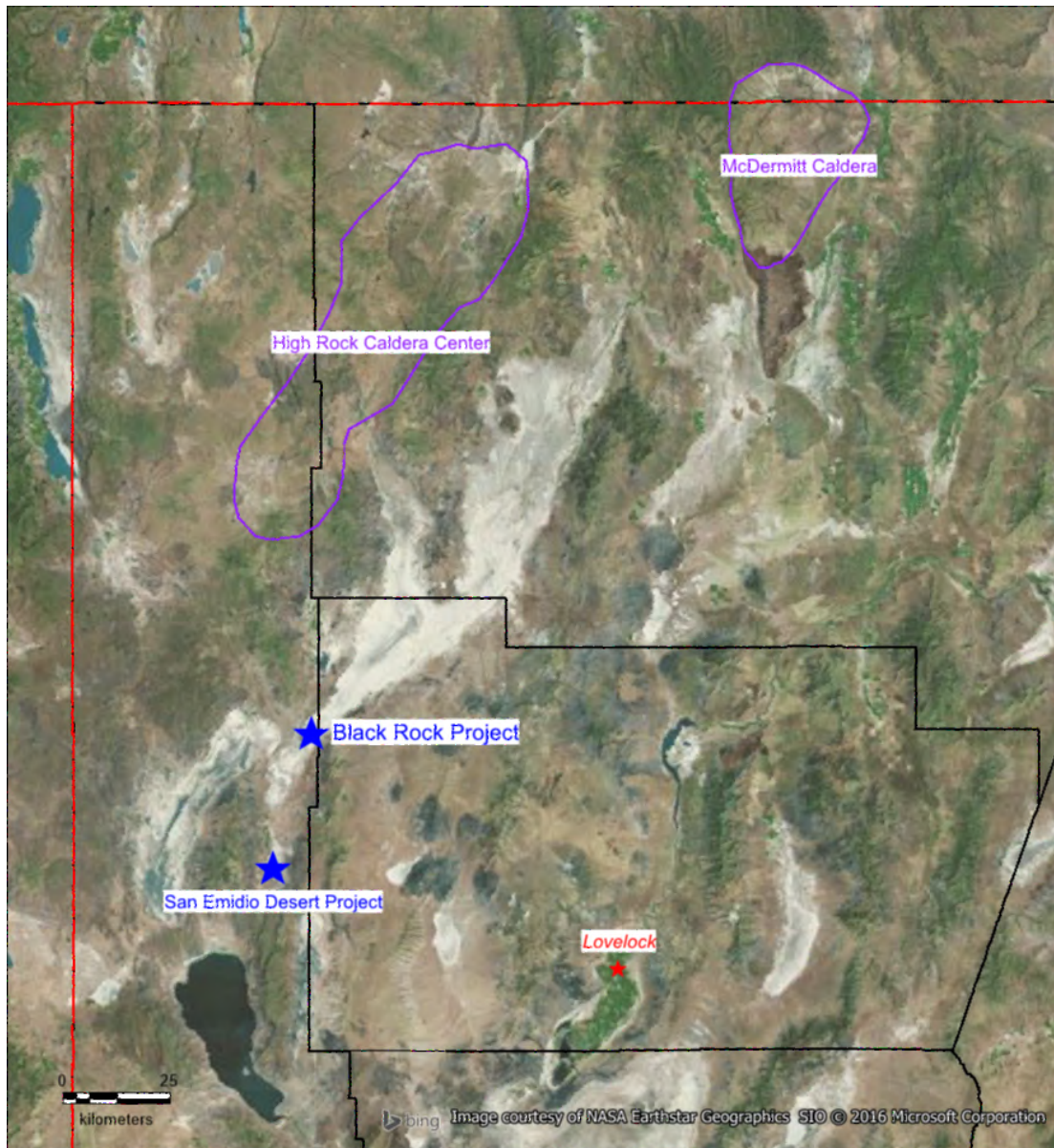
Figure 6 Calderas in the Black Rock Desert region
