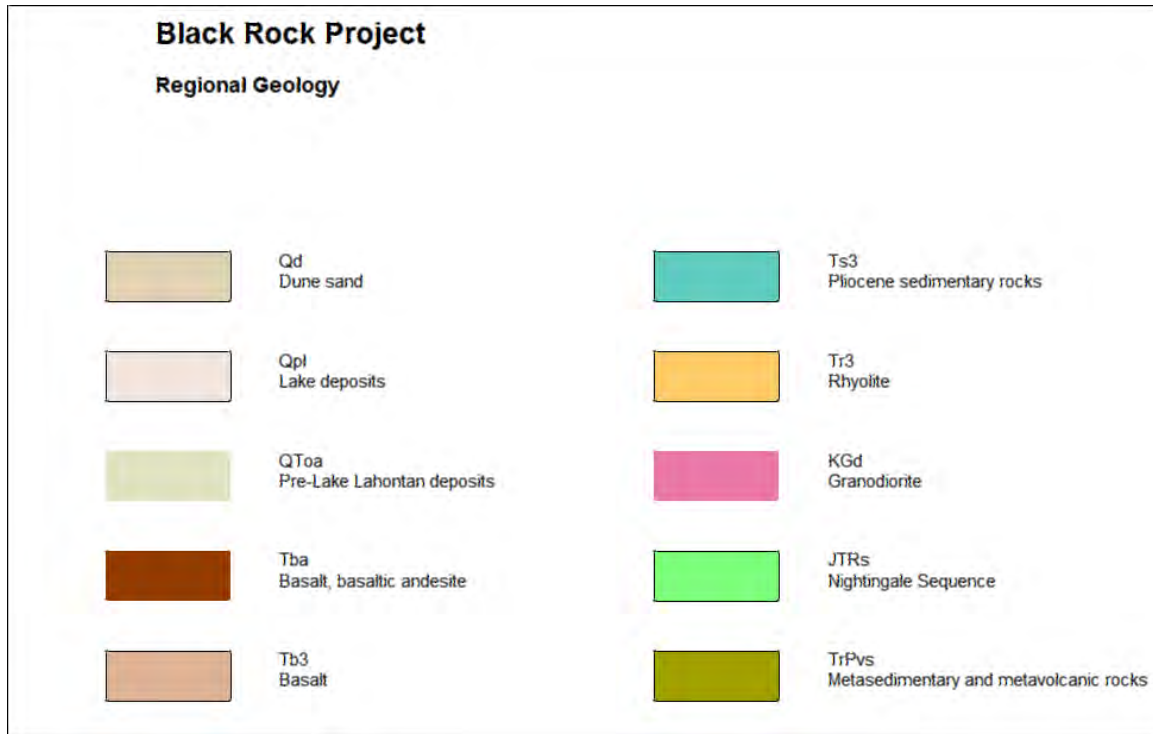
Figure 8 Black Rock Desert Project Generalized Geologic Units
