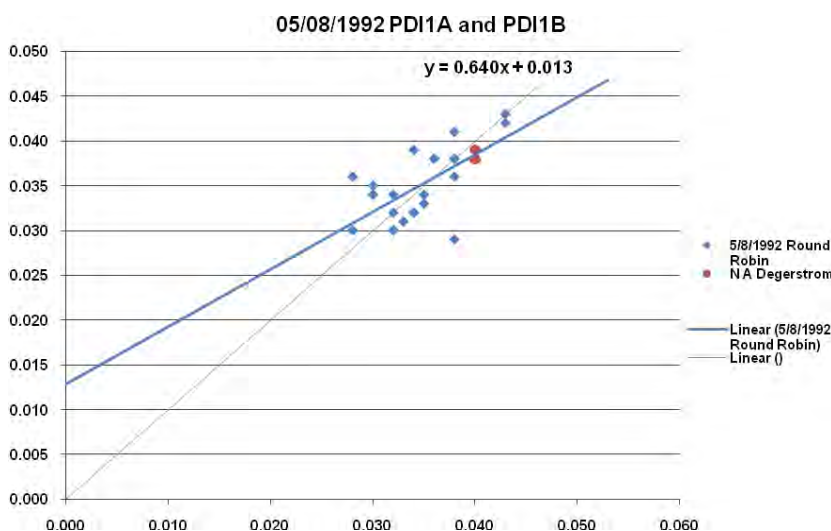
Figure 16.2A Round Robin Analysis Results for Samples PDI1A and PDI1B (05/08/92)
