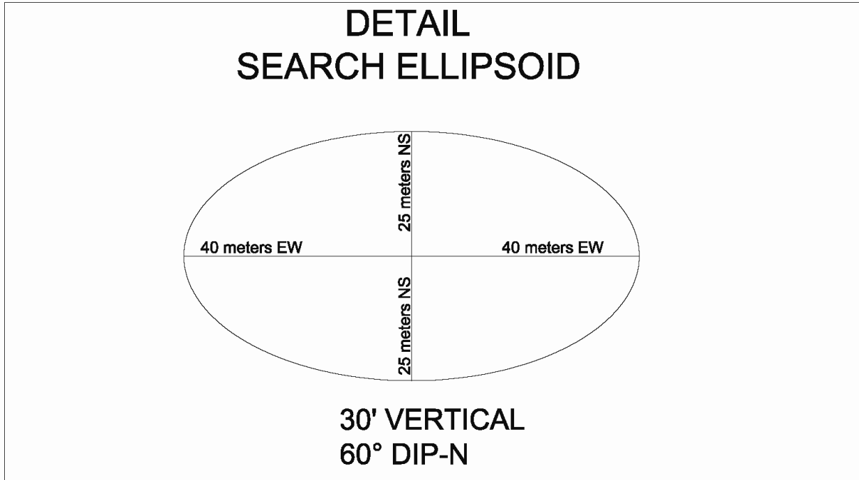
Figure 19.15 Search Orientations for the Bell Mountain Block Model
