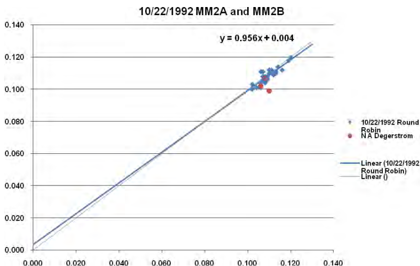
Figure 16.4B Round Robin Analysis Results for Samples MM2A and MM2B (10/22/92)
