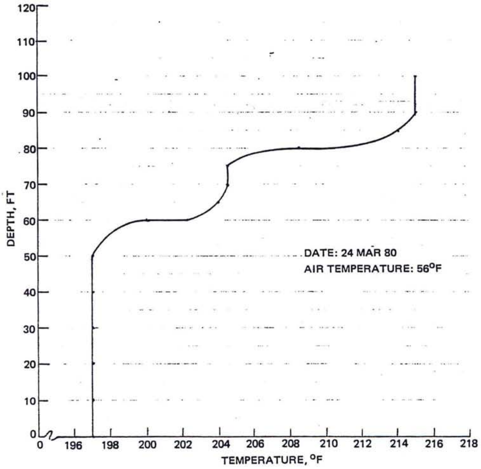
FIGURE 28. Temperature Log, Well 4K-1.
