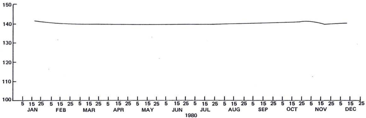
FIGURE 22. Coso Well 1 Water Level.
