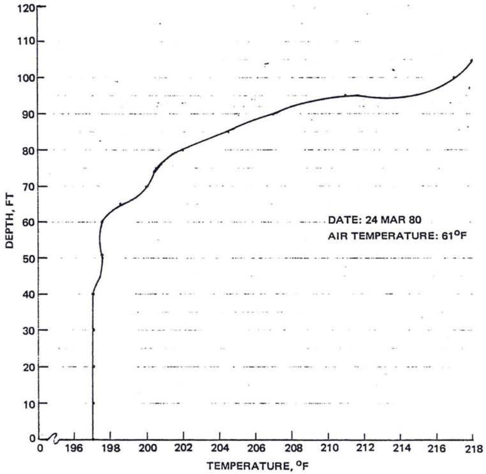
FIGURE 27. Temperature Log, Well 4P-1.
