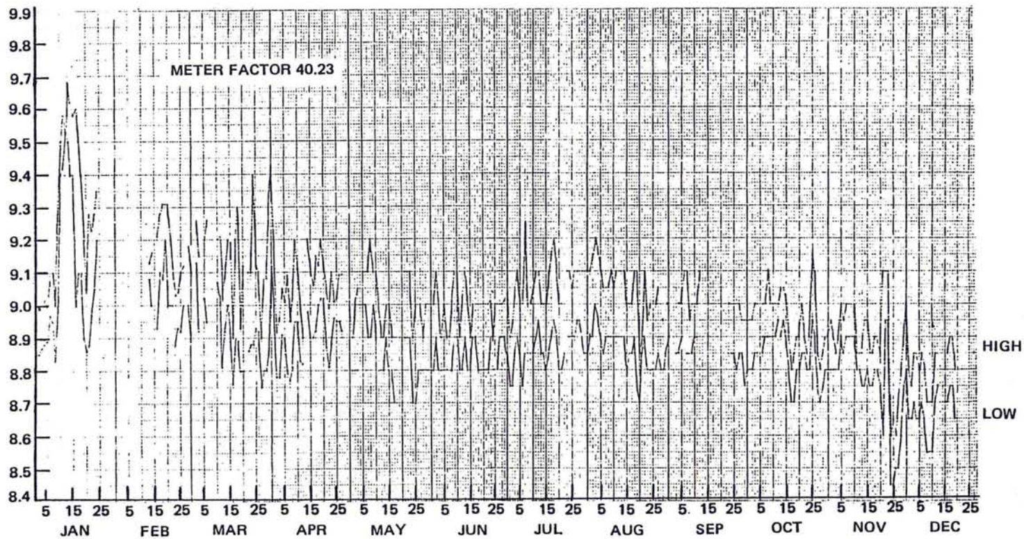
FIGURE 2. Devils Kitchen Steam Flow Meter Values, 1980.
