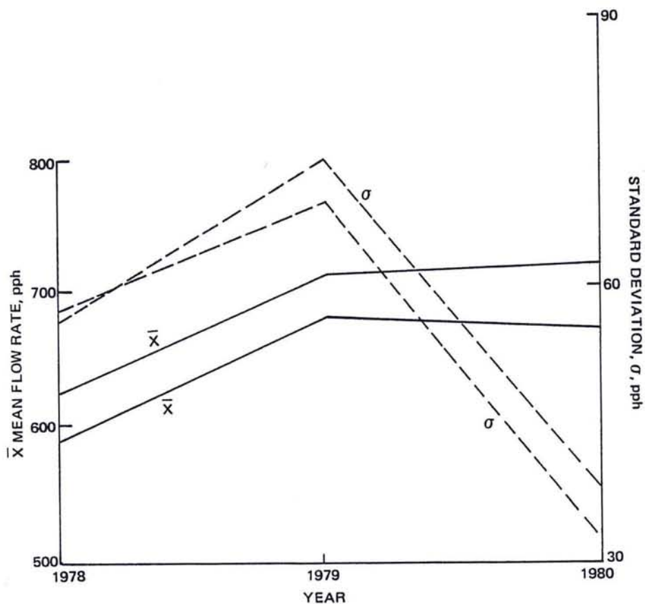
FIGURE 5. Coso Corrosion Array Statistical Steam Flow Data.
