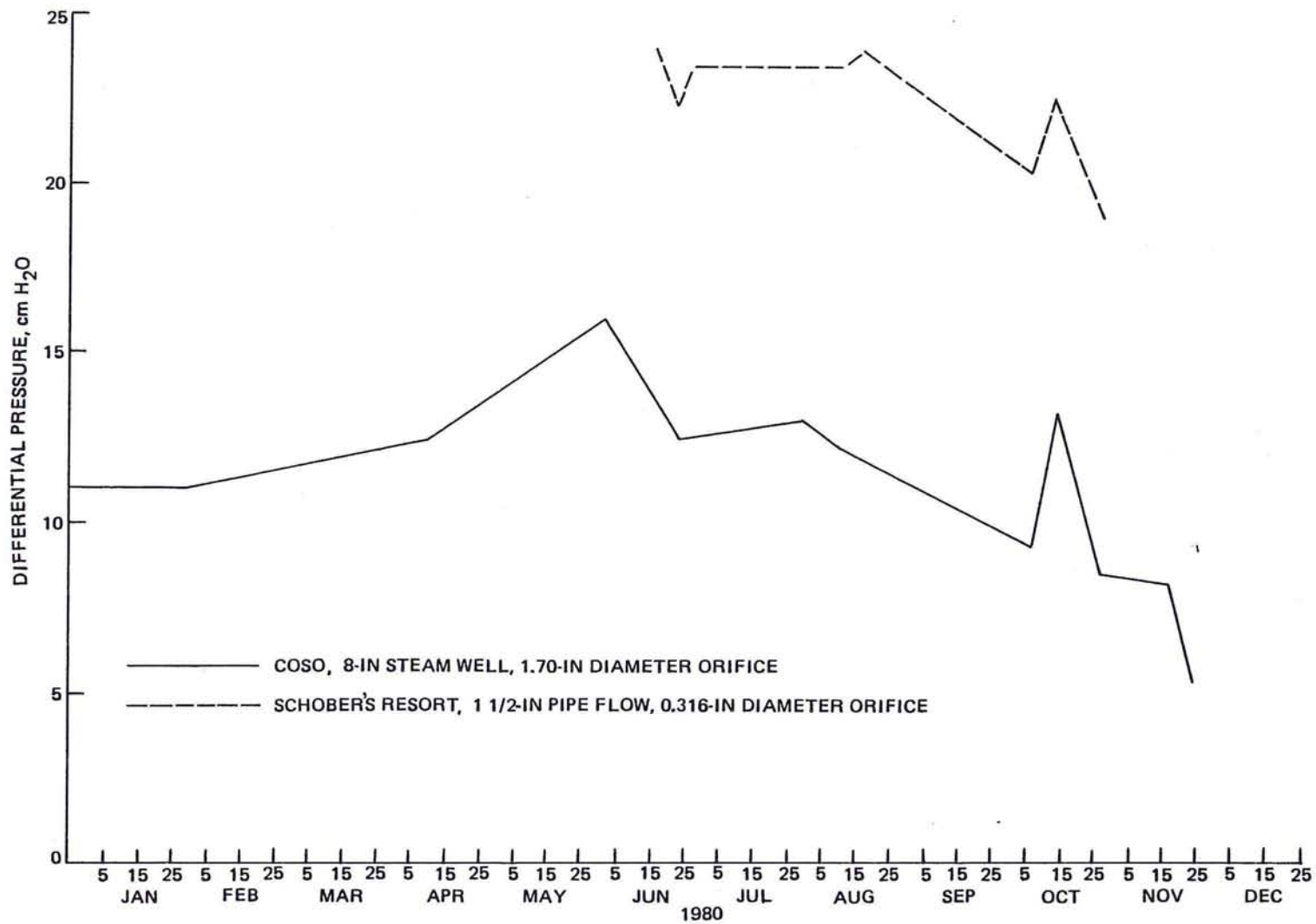
FIGURE 8. Steam Flow Monitoring at Coso With Manometer.
