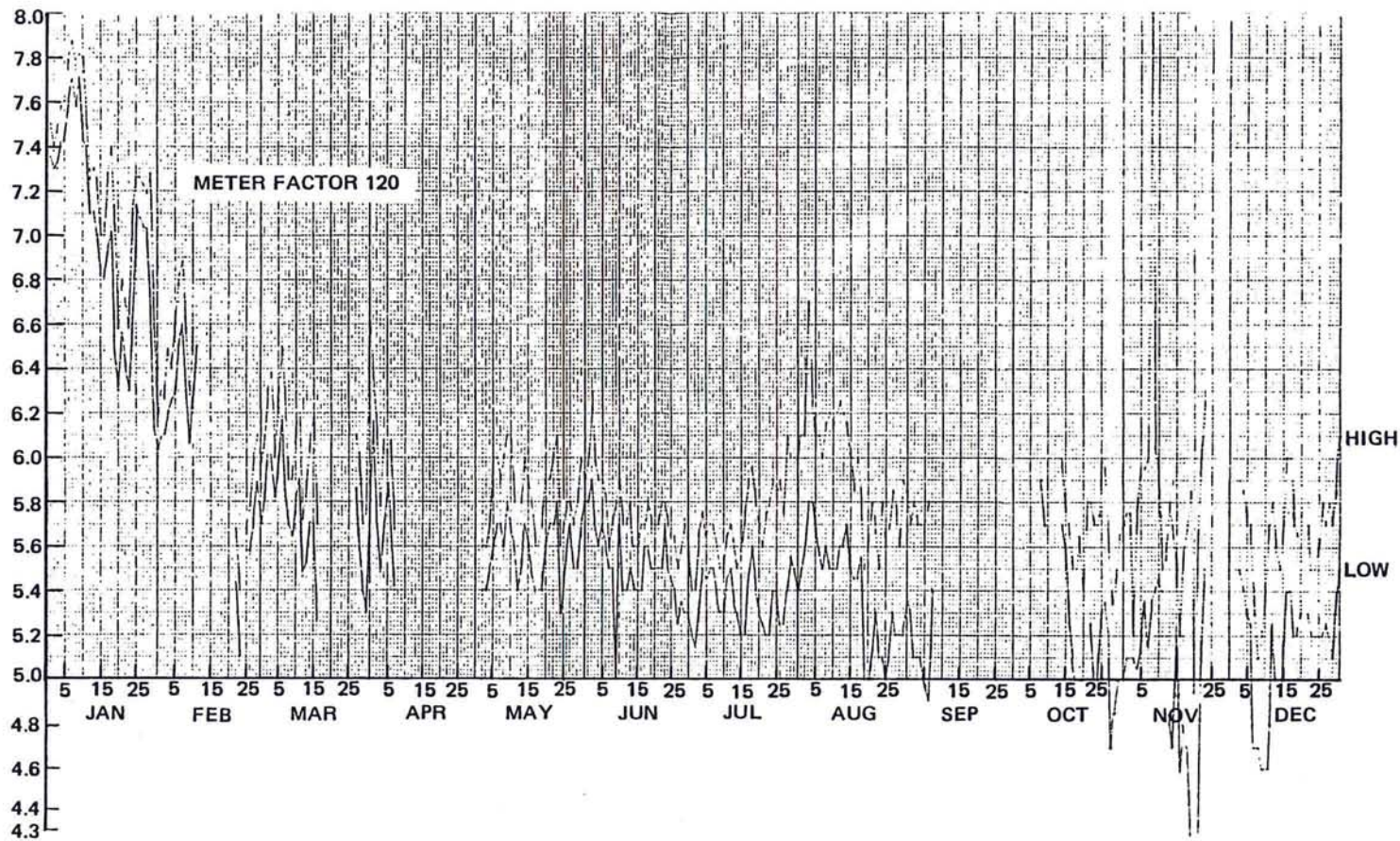
FIGURE 4. Coso Corrosion Array Steam Flow Meter Values, 1980.
