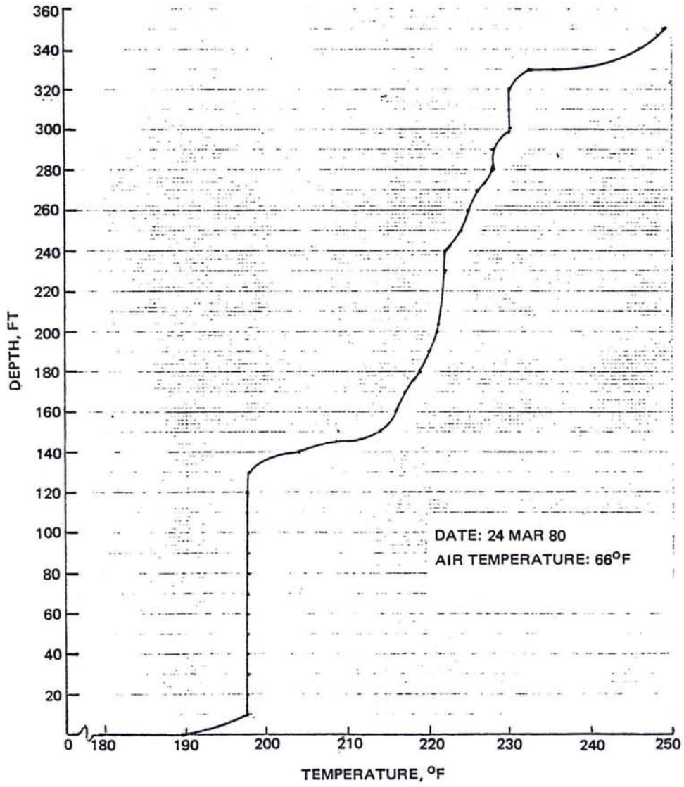
FIGURE 26. Temperature Log, Coso Well 1.
