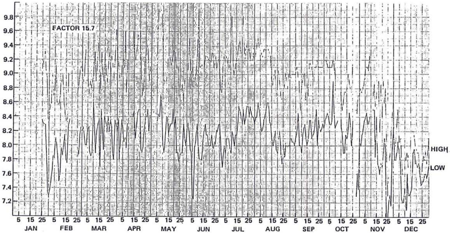
FIGURE 6. Coso No. 2 Steam Flow Meter Values, 1980.
