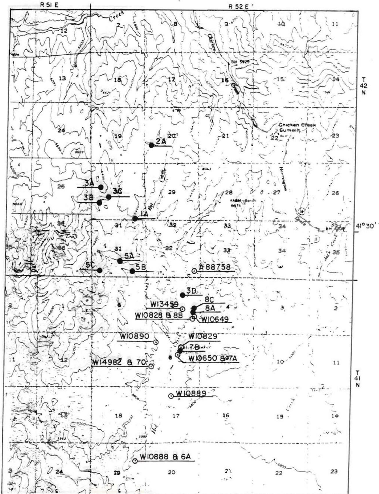
○ AMAX Figure 5. Location map for hydrogeochemical samples at the Tuscarora project. ● UURI
