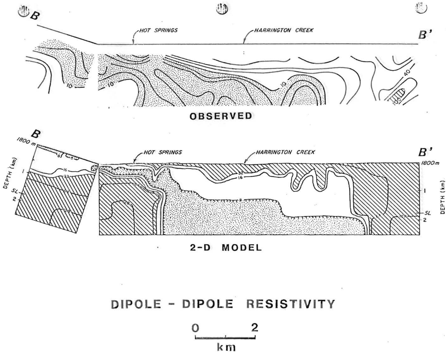
Figure 12. Resistivity sections along line B-B' showing observed and modelled resistivity.
