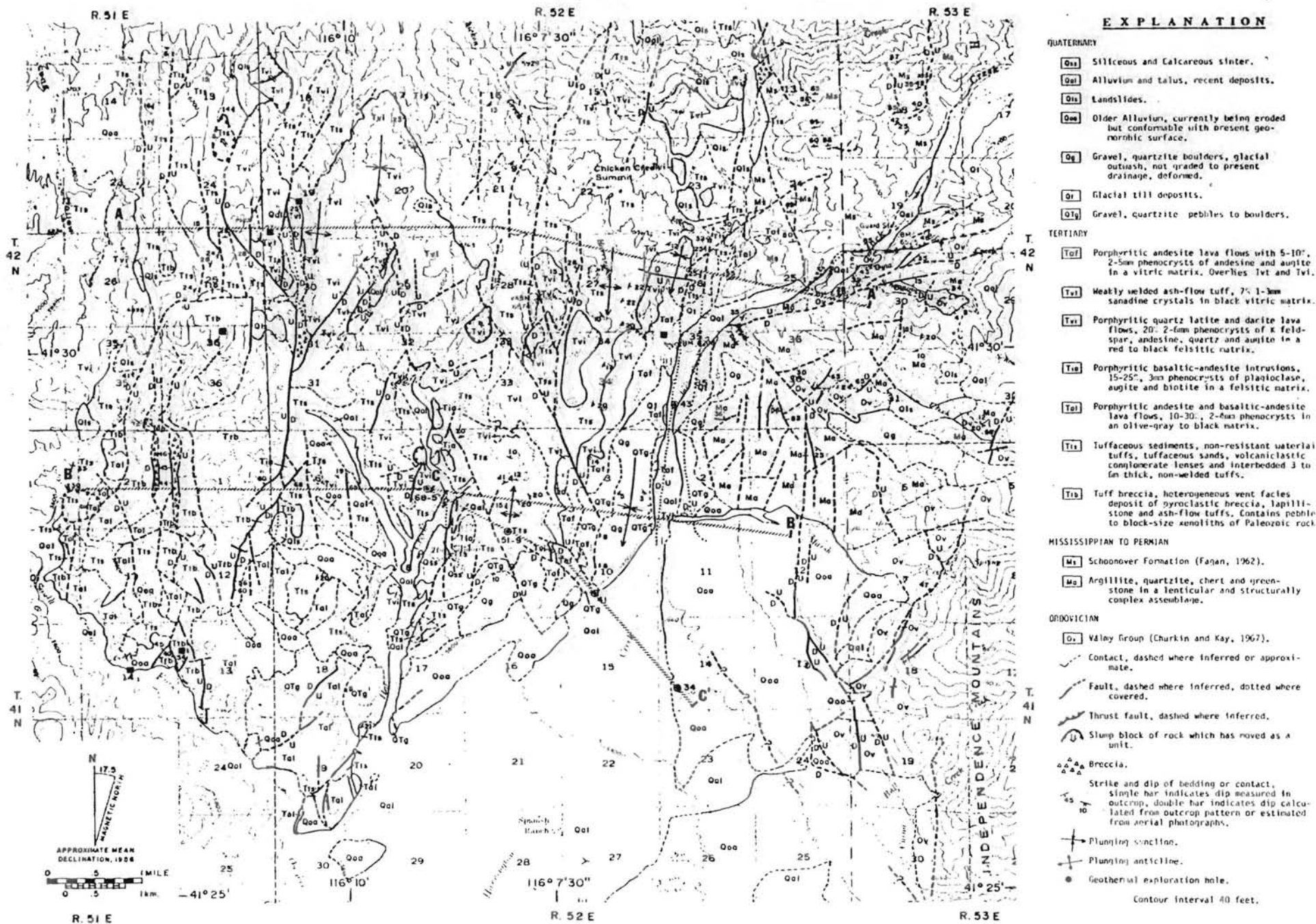
Figure 2. Geologic map of the Tuscarora area, Nevada after Sibbett (1980) Mapping done under DOE contract DE-AC07-80IN12079
