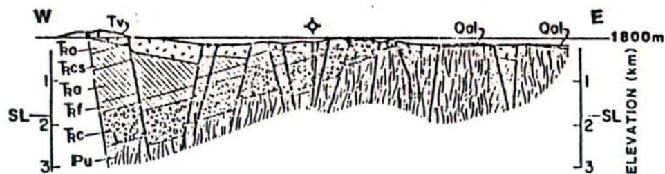
Figure 11. Gravity profile with automatic interpretation for densities (top) after Berkman (1930) compared with geologic cross-section (bottom) after Pilkington, 1980.
