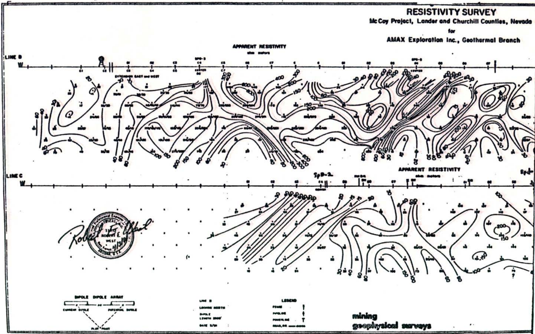
Figure 17. Resistivity survey McCoy Project, Nevada Line B and C
