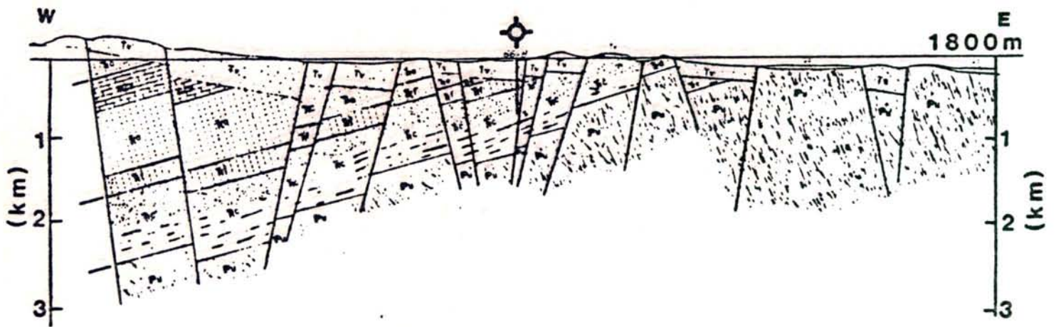
Figure 3. Geologic cross-sections through well 14-7 (Top) and well 66-8 (bottom) after Pilkington, 1980.
