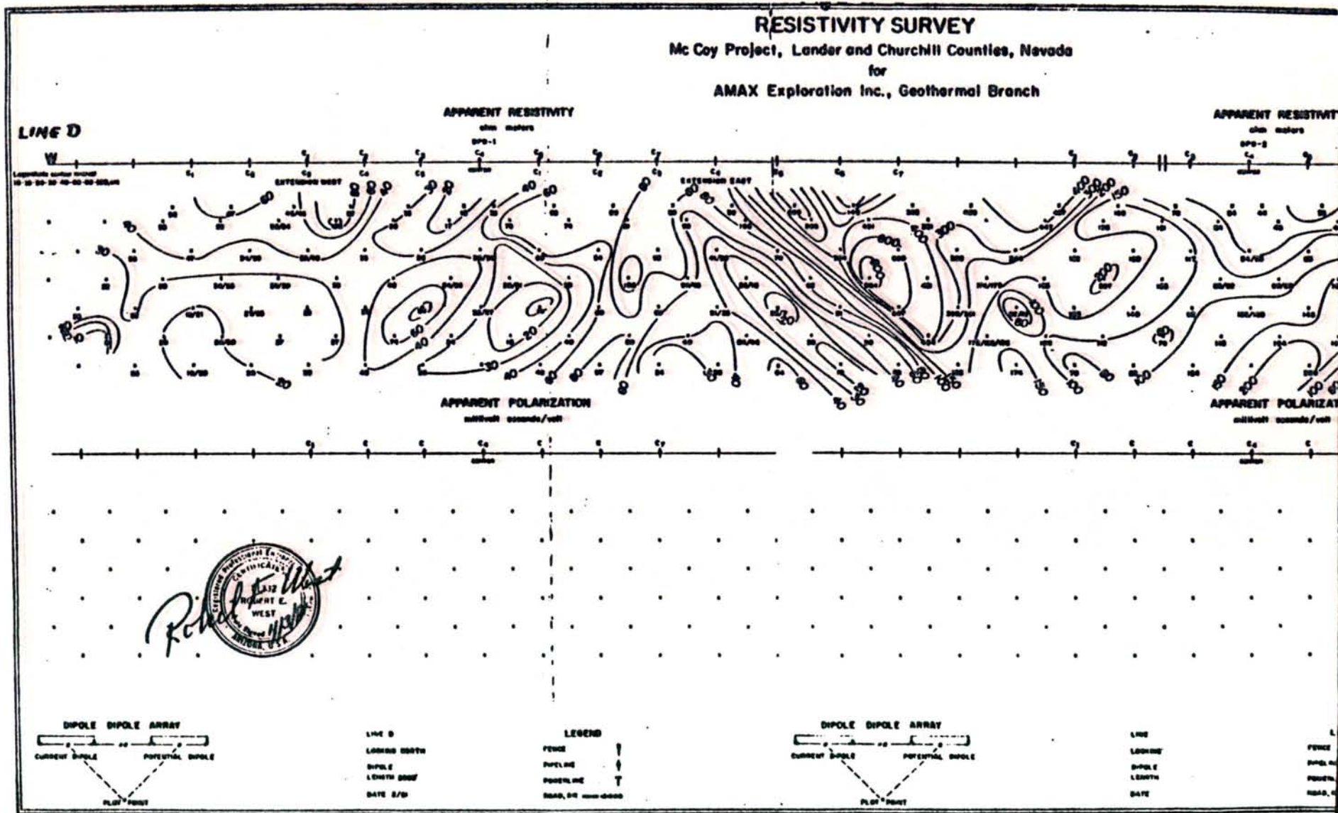
Figure 18. Resistivity survey McCoy Project, Nevada Line D
