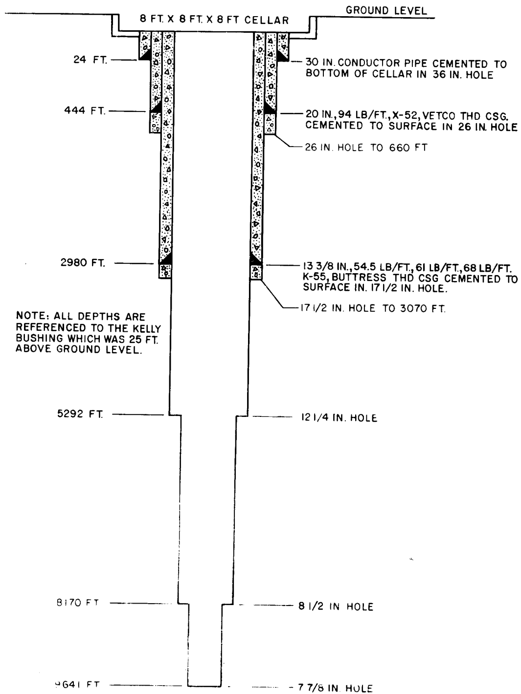
DESERT PEAK WELL NO. B-23-1 SUBSURFACE WELL PROFILE
