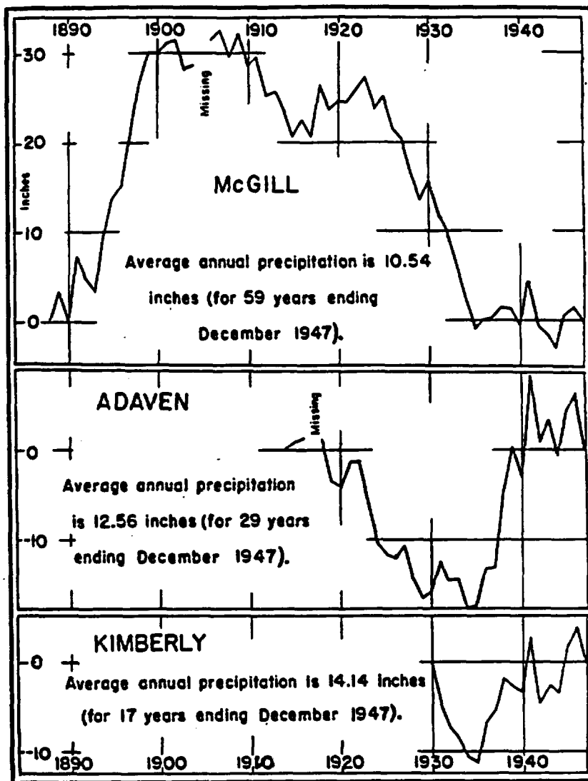
FIGURE 2—Graphs showing cumulative departure from average annual precipitation at three stations in eastern Nevada.
