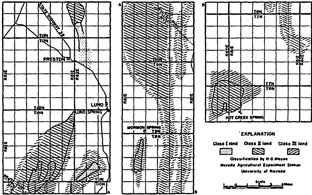
FIGURE 5—Reconnaissance classification of land in White River Valley, Nevada.
