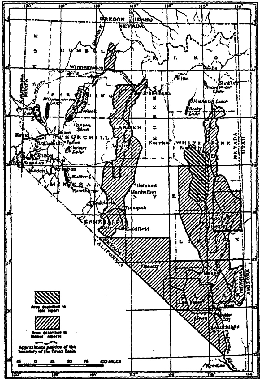
FIGURE 1—Map of Nevada showing areas covered by published ground-water reports and by the present report.
