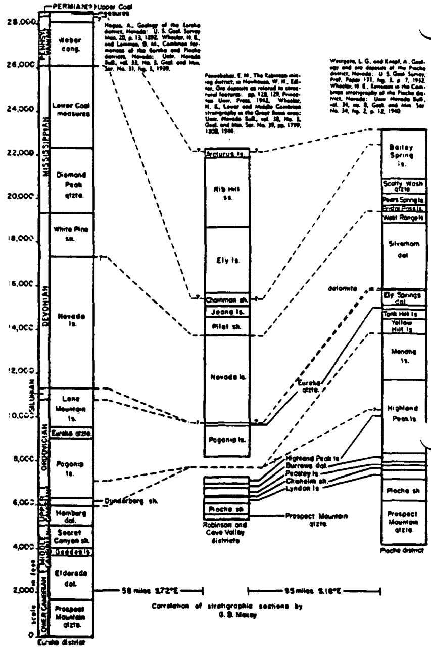
FIGURE 3—Diagrammatic correlation of Paleozoic stratigraphic columns in the Eureka, Pioche, and Robinson mining districts, and Cave Valley, Nevada.
