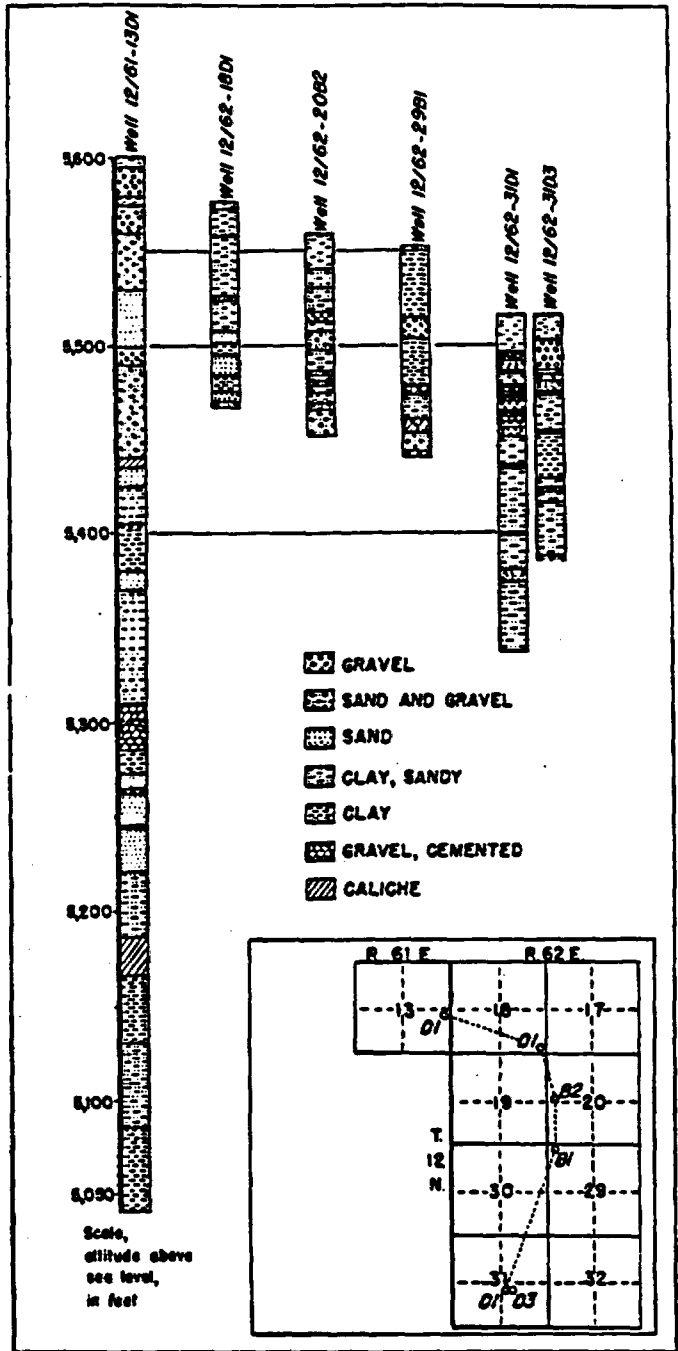
FIGURE 4—Selected logs of wells in White River Valley, Nevada.
