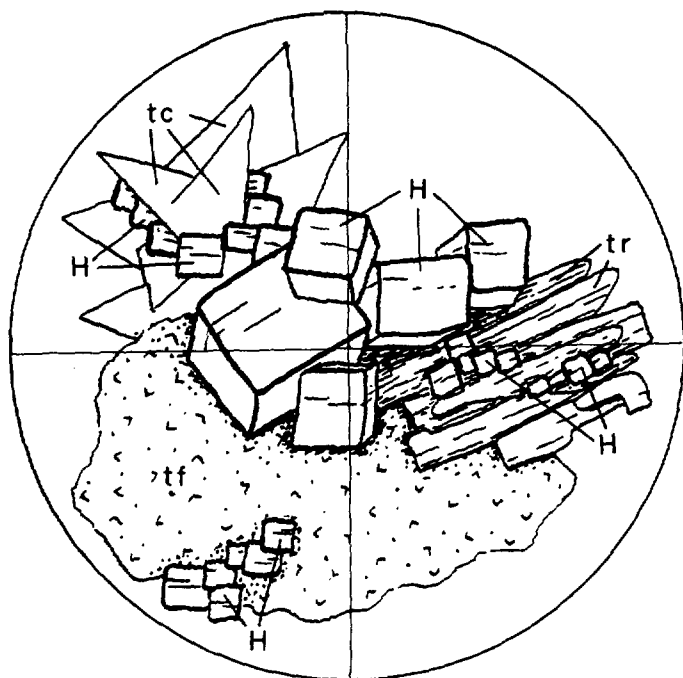
FIGURE 24.—Micrograph of powdered salts from efflorescence in marshes in the carbonate zone. The chief salts are sodium carbonate, trona or thermonatrite (tr); a coarsely crystalline (tc) and finely crystalline (tf) form of sodium sulfate, thenardite; and sodium chloride, halite (H). The halite is the last to crystallize and grows over and around the other minerals. The finely crystalline thenardite, which probably includes other minerals, commonly forms a pedestal on which the coarse thenardite and trona have grown, as if it were the earliest of the minerals to form. Diameter of field, 0.5 mm.
