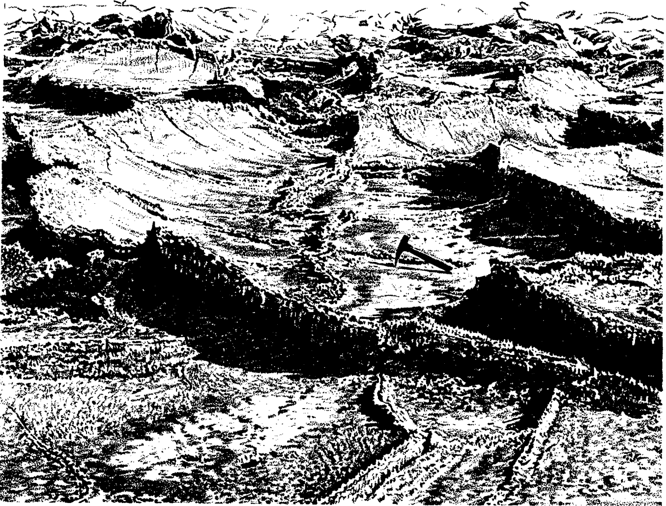
FIGURE 57.—Salt saucers west of Badwater. Drawn by John R. Stacy, from photograph.
