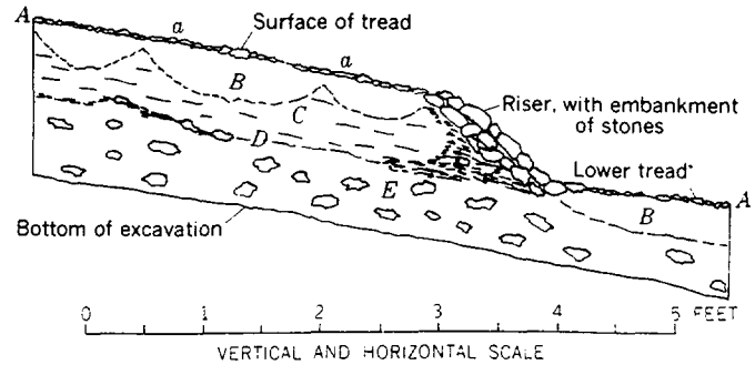
FIGURE 66.—Section of sorted step. A , Pavement of fine pebbles on tread of sorted step. a , Locations of salt efflorescence on tread. B , Dry porous light-gray layer cemented by salts; some stones. C , Damp soft brown layer with reddish spots; rises to within 0.5 inch of surface under spots of salt efflorescence. D , Firmly cemented stony layer. E , Parent gravel, not well cemented.
