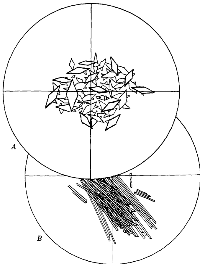
FIGURE 22.—Micrographs of gypsum crystals from the sulfate layer in the silt facies of the carbonate zone. The gypsum occurs in nodules which in part are aggregates of nearly diamond-shaped crystals (A) and in part are straight fibers (B). Diameter of fields, 0.5 mm.
