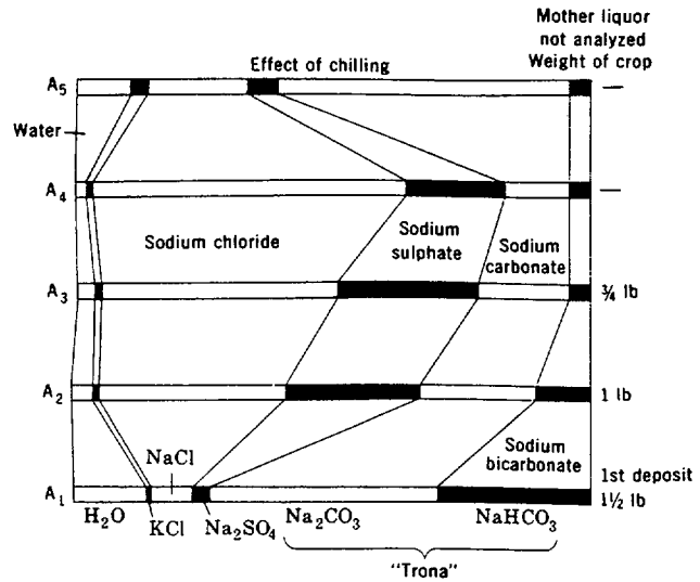
FIGURE 52.—Diagram illustrating graphically the results of Chatard's experiments with the evaporation of water from Owens Lake, Calif. A 1 to A 4 are the successive crops of salts obtained by Chatard as a result of evaporation of the brine at temperatures in the range of 77° to 96°F; A 5 is the crop obtained by chilling the remaining liquid of A 4 to 57°F. Adapted from Gale, 1915, fig. 75.
