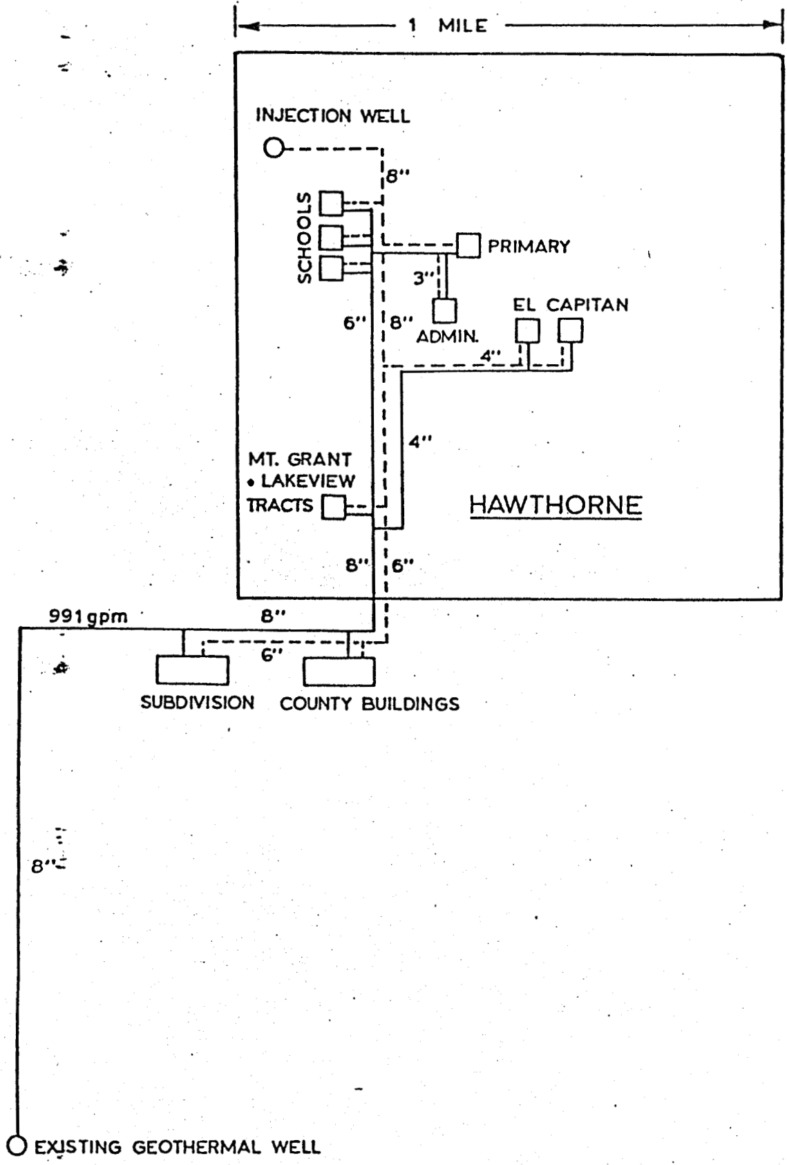
FIGURE 4.1 Alternate I plot plan (from Geo-Heat Utilization Center, 1981).
