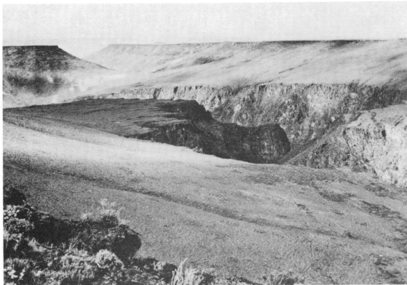
FIGURE 8.—Double canyon of Virgin Creek south of Virgin Valley, Charles Sheldon Wilderness Study Area. Photographer was standing on rim of upper part of rhyolite of Badger Mountain looking northeast; below him is slope underlain by tuffaceous sedimentary rocks and below that is inner canyon cut in lower part of rhyolite of Badger Mountain. Across canyon, slope is of tuffaceous sedimentary rocks capped by basalt of Rock Spring Table.
