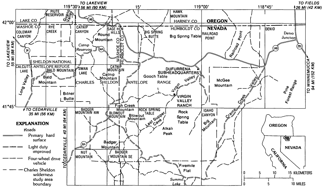
FIGURE 1—Map showing location and geographic features of the Charles Sheldon Wilderness Study Area, Humboldt and Washoe Counties, Nev, and Lake and Harney Counties, Ore
