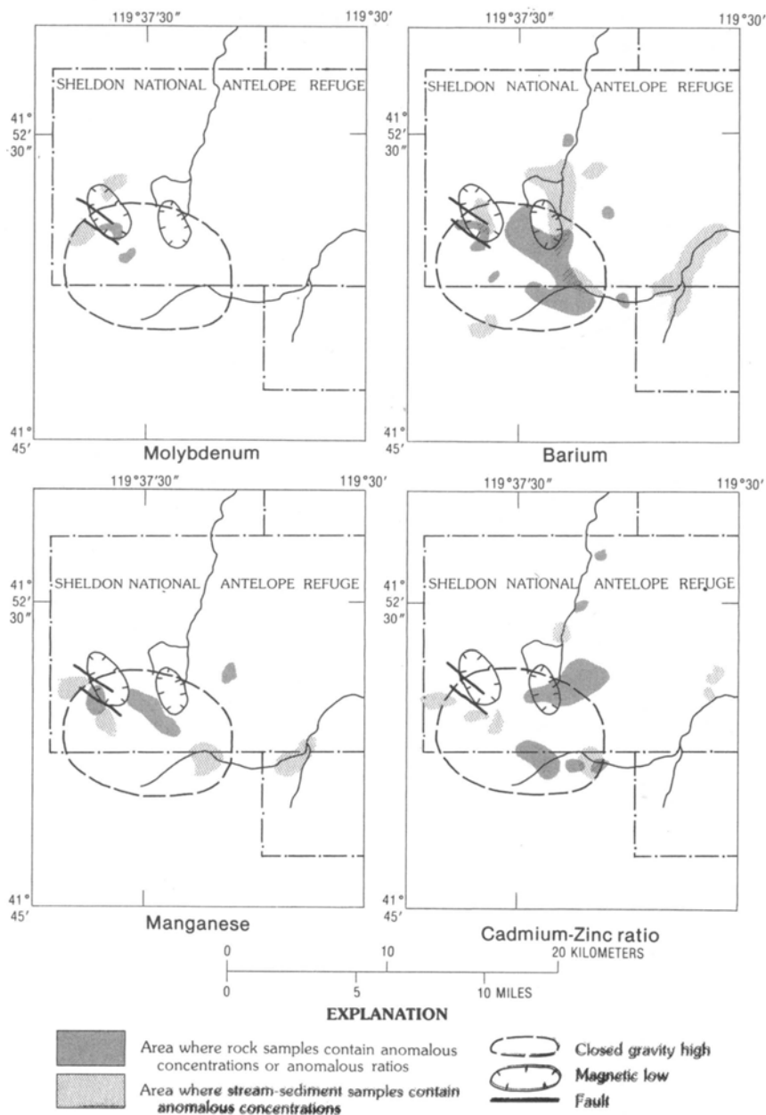
FIGURE 13. —Relationship between selected aeromagnetic lows, faults, a gravity high, and anomalous concentrations of molybdenum, barium, and manganese, and anomalous cadmium:zinc ratios \geq 0.05 in rock and stream-sediment samples in the Lone Pine district, Charles Sheldon Wilderness Study Area. Method of analyses: Mo, Ba, and Mn by emission spectroscopy; Cd and Zn by atomic absorption. Analyst: E. F. Cooley, G. L. Crenshaw, and D. F. Siems.
