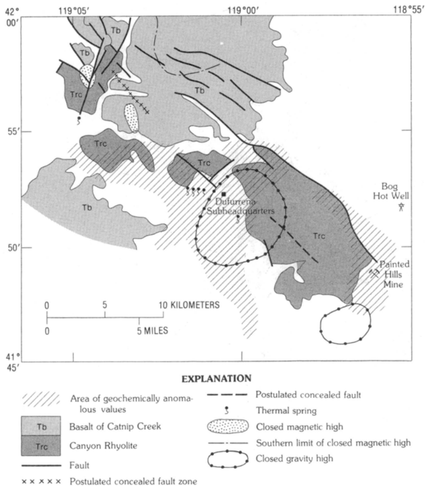
FIGURE 23.—Relationship of geochemically anomalous areas of the Painted Hills mine and Subheadquarters, Charles Sheldon Wilderness Study Area.
