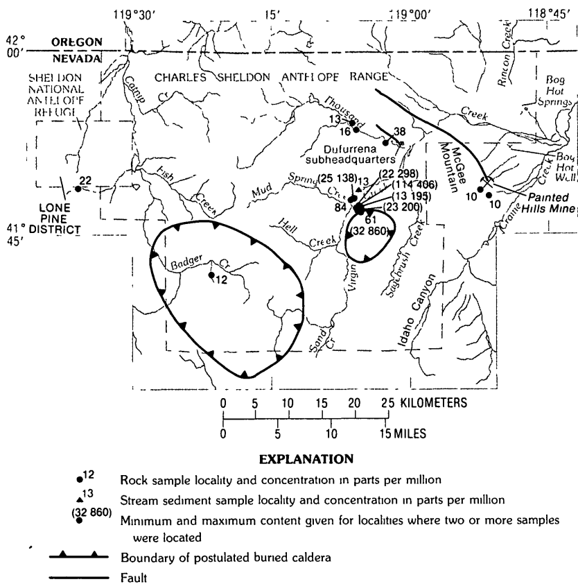
FIGURE 26 —Distribution of uranium \geq 10 ppm in rock and stream-sediment samples, Charles Sheldon Wilderness Study Area Analytical method neutron activation Analyst H L Millard, Jr , and R J Knight
