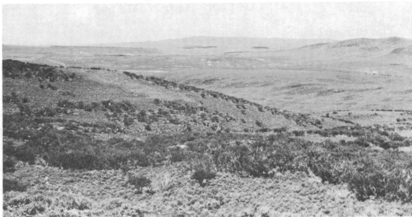
FIGURE 6.—View north from Badger Mountain, Charles Sheldon Wilderness Study Area. Foreground underlain by rhyolite of Badger Mountain. In middle distance Badger Creek valley underlain by tuffaceous sedimentary rocks with local basalt caps; right side is Fish Creek Mountain underlain by rhyolite of Badger Mountain. Far distance in center is Catnip Mountain, underlain by rhyolite of Catnip Mountain. Extreme distance on left, Hart Mountain.
