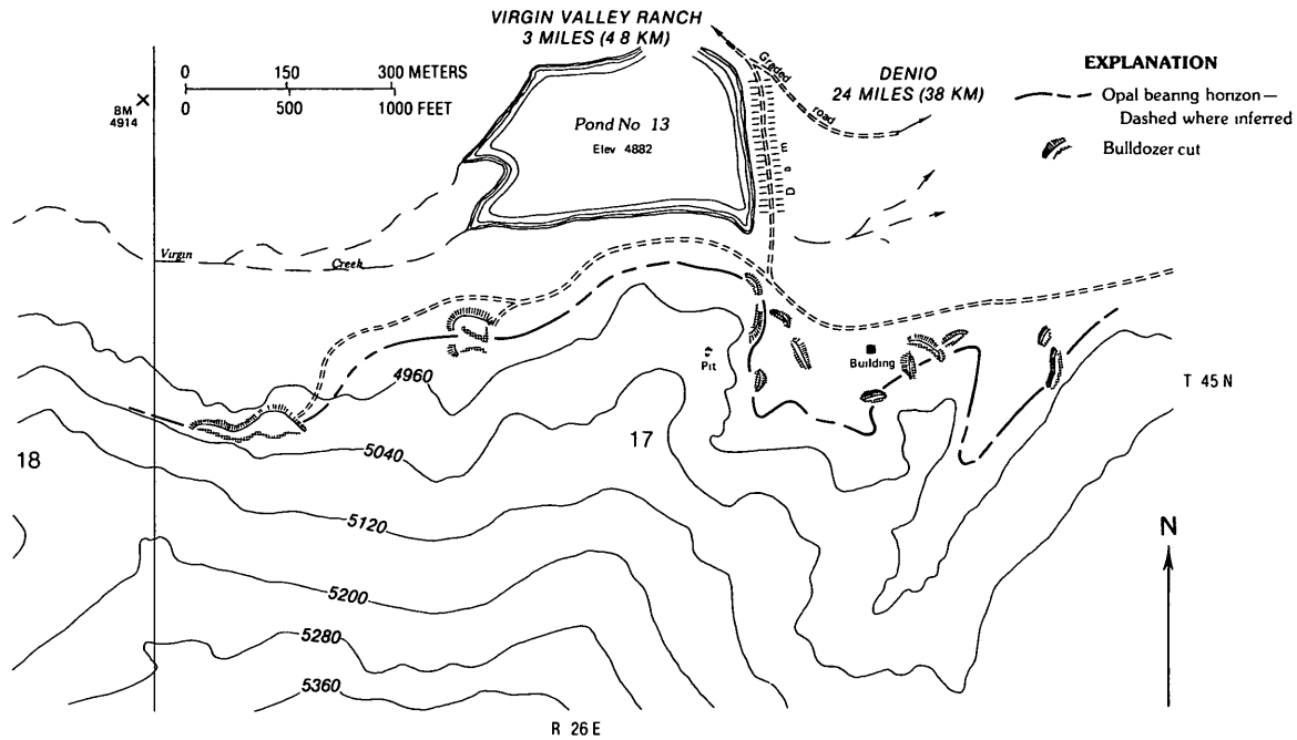
FIGURE 31 —Meyer group mine workings, Charles Sheldon Wilderness Study Area
