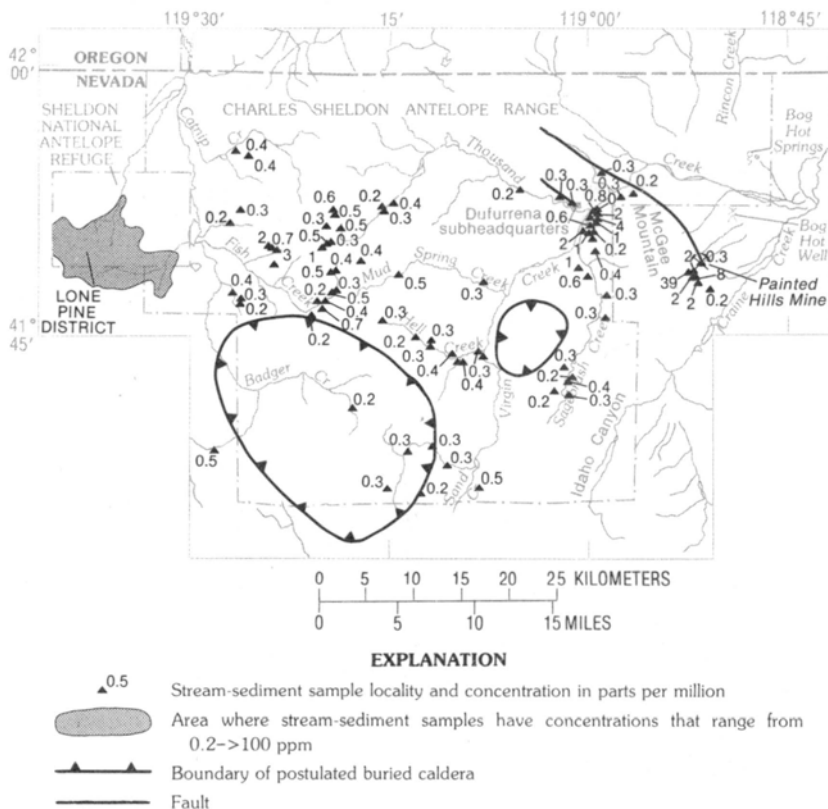
FIGURE 15.—Distribution of anomalous concentrations of mercury in stream-sediment samples, Charles Sheldon Wilderness Study Area. Analytical method: flameless atomic absorption. Analyst: G. L. Crenshaw.
