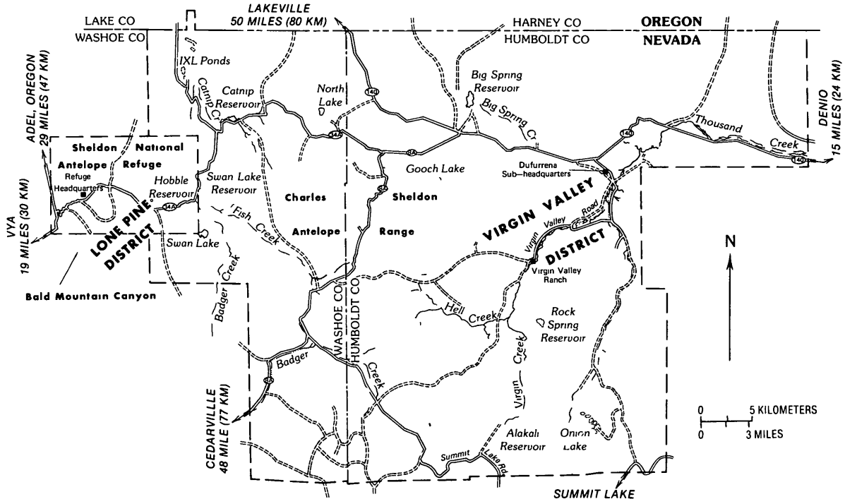
FIGURE 27 —Map showing mining districts, Charles Sheldon Wilderness Study Area
