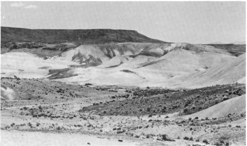
FIGURE 9.—Bedded tuffaceous sedimentary rocks, about 0.6 mi (1 km) south of Thousand Creek Spring, Charles Sheldon Wilderness Study Area. Badlands topography here contains many opal claims. Big Spring Table in background; basalt caps sedimentary rocks. Two levels separated by normal fault. View to the north.
