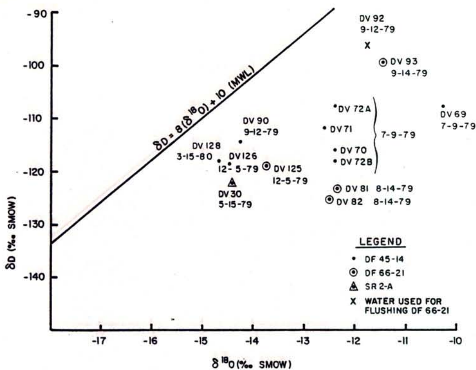
Figure H-8. Deuterium and Oxygen-18 Compositions of Deep Wells DF45-14 and DF66-21.
