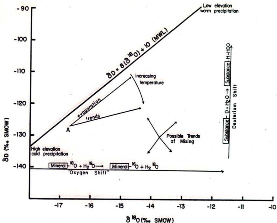
Figure H-1. General Principles of Stable Isotope Data Interpretation.
