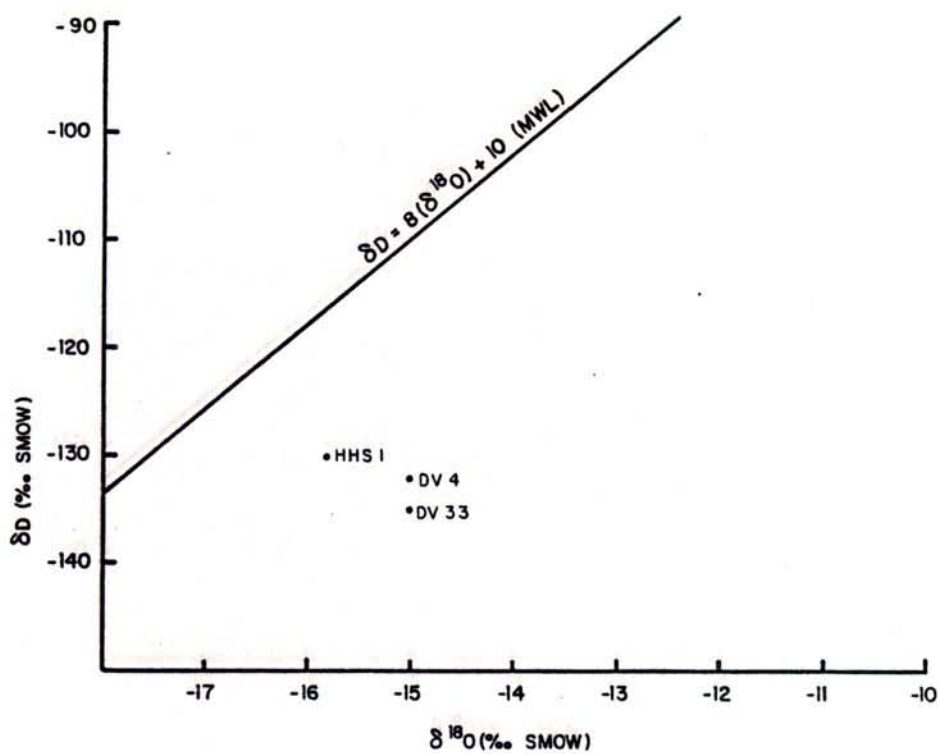
Figure H-3. Deuterium and Oxygen-18 Compositions of Hyder Hot Springs.
