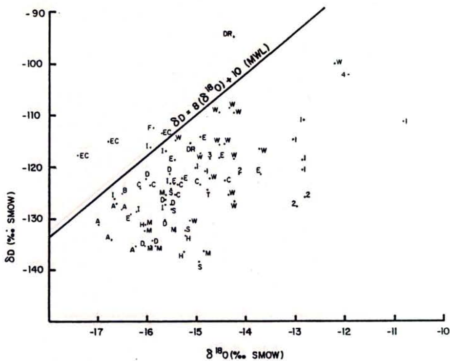
Figure H-10. Deuterium and Oxygen-18 Compositions of Dixie Valley and Surrounding Waters.
