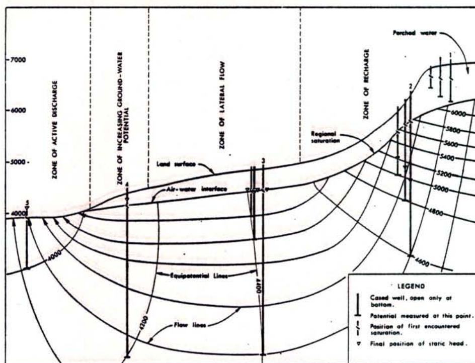
Figure H-11. Sketch of Observed Relationship in a Typical Desert Basin Flow System (after Mifflin, 1968)
