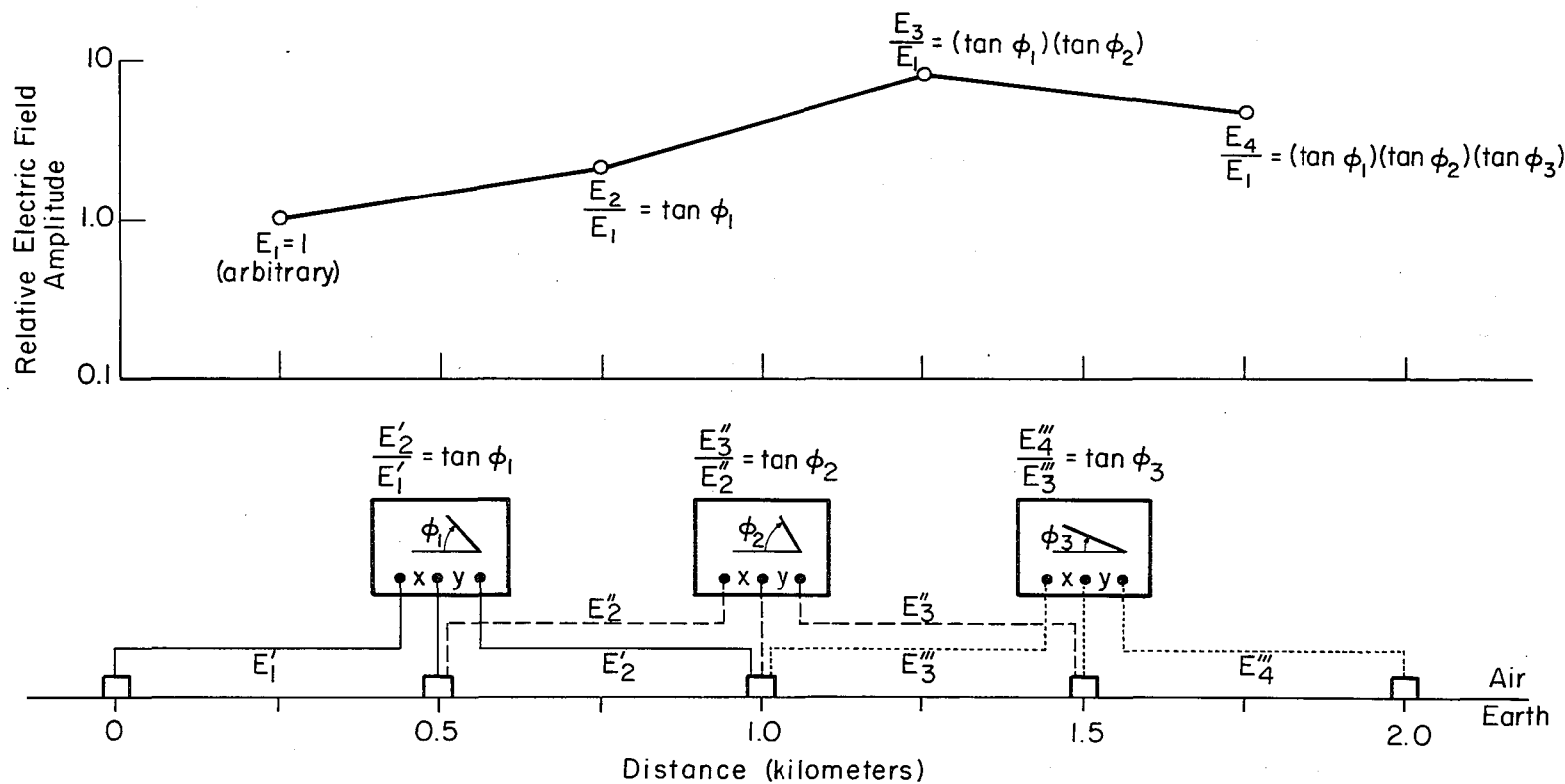
Figure I-3. Three successive E-field ratio telluric receiver stations and data plotting method.
