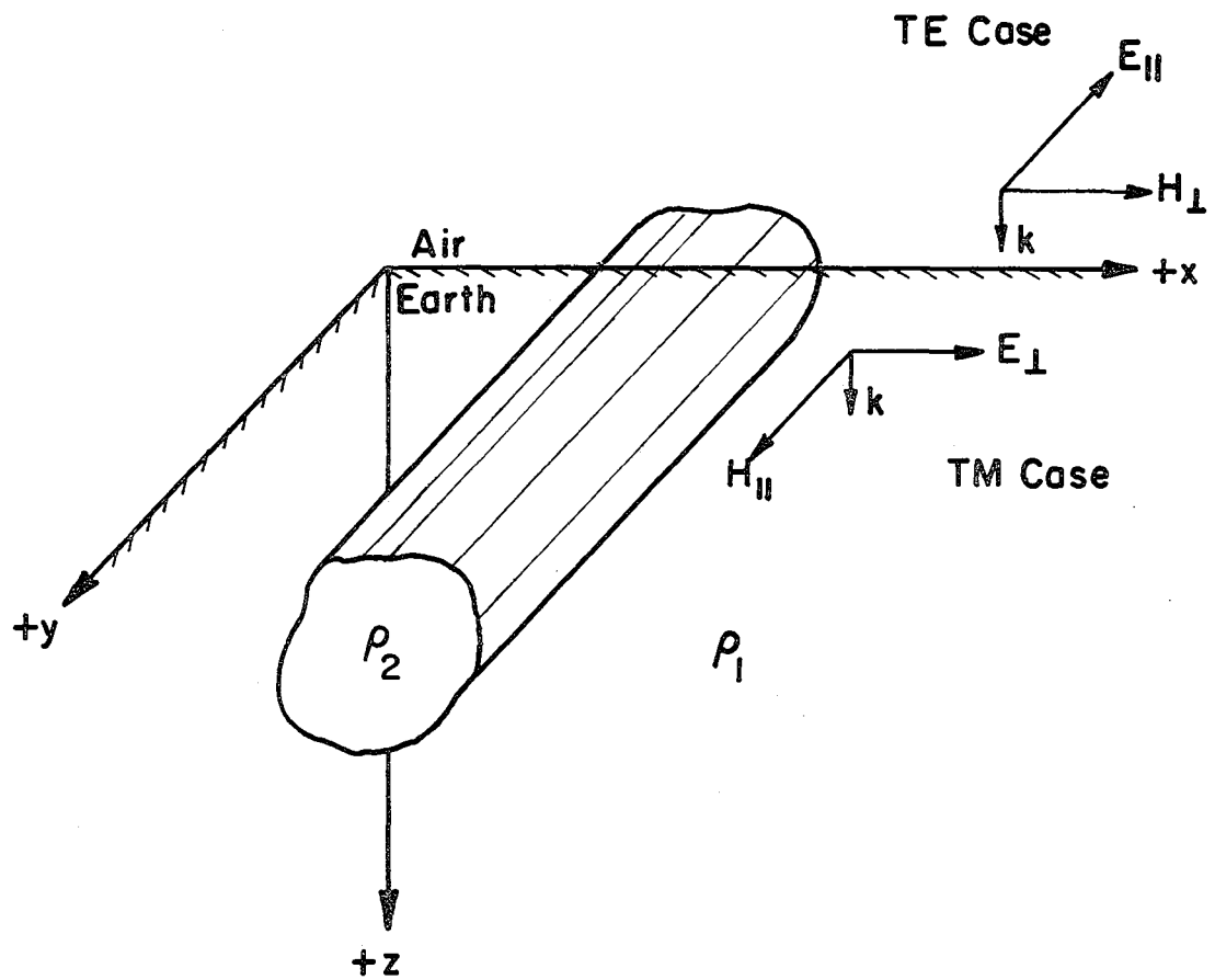
Figure I-1. Coordinate system containing a two-dimensional resistivity inhomogeneity, and showing transverse electric and transverse magnetic field directions.
